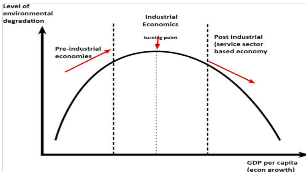
Figure 3.1 EKC Hypothesis.
