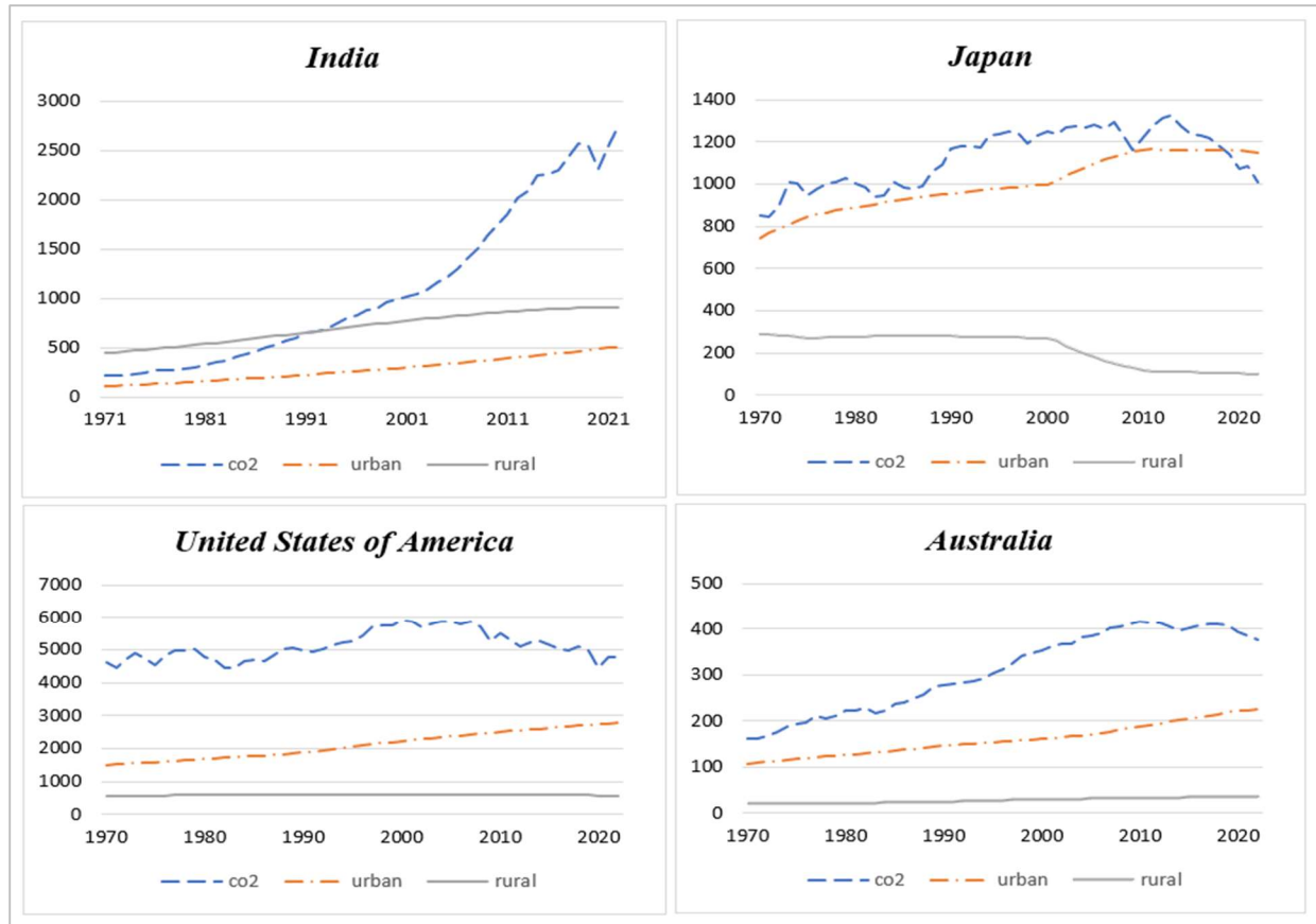
Figure 5.2 Trend of CO 2 emissions, urban, and rural population of QUAD nations.
