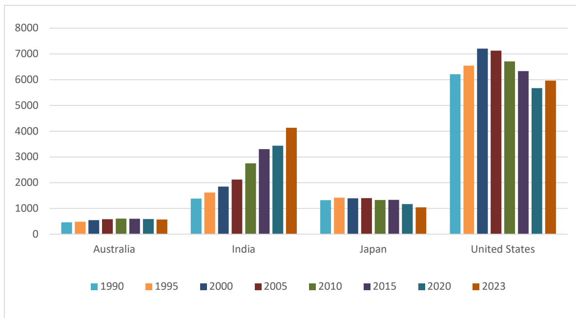
Figure 2.4 GHG emissions of QUAD nations from the year 1990 to 2023.
