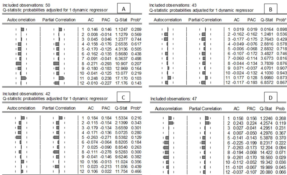
Figure 5.22 Autocorrelation test results for QUAD nations.
