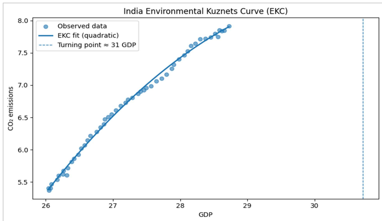
Figure 5.18 EKC for India. Source: Computed by the authors.
