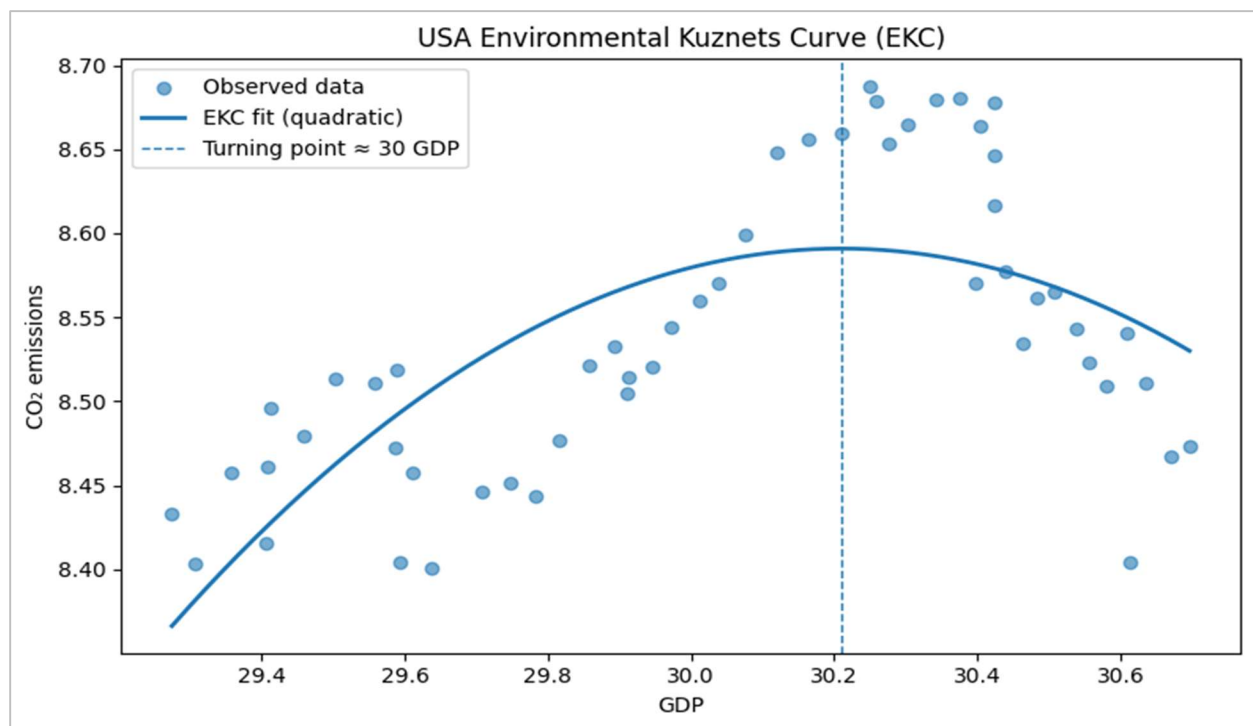
Figure 5.19 EKC for the USA. Source: Computed by the authors.
