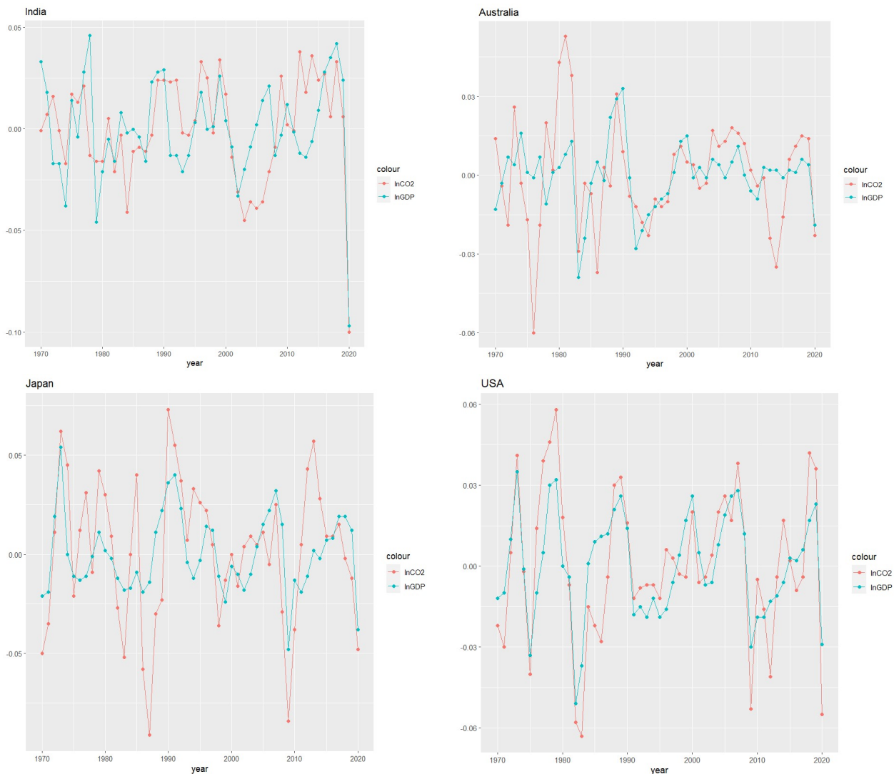
Figure 5.6 Co-Movement of CO 2 emissions and GDP cycles. Source: Computed by the authors.
