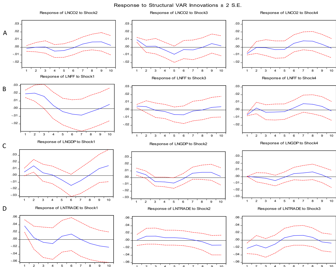
Figure 5.10 Structural Impulse Response Function with one innovation shock in CO 2 emissions for India.
