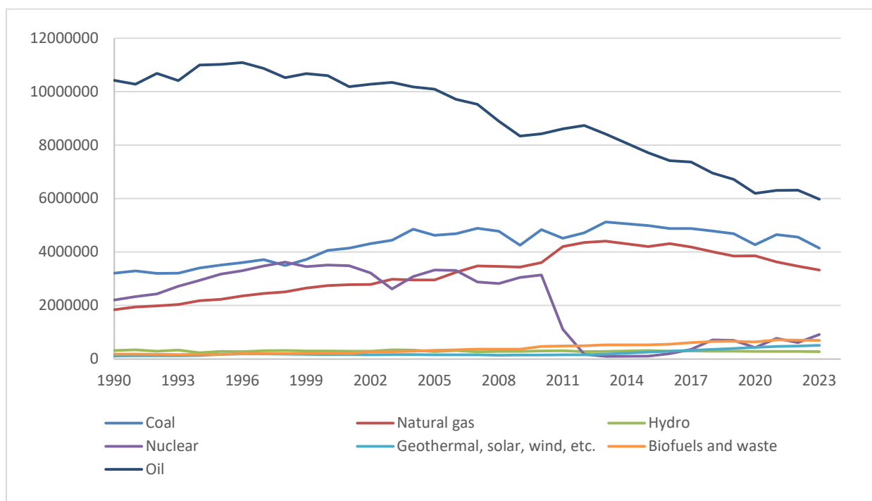
Figure 2.5 Energy basket of Japan from the year 1990 to 2023.
