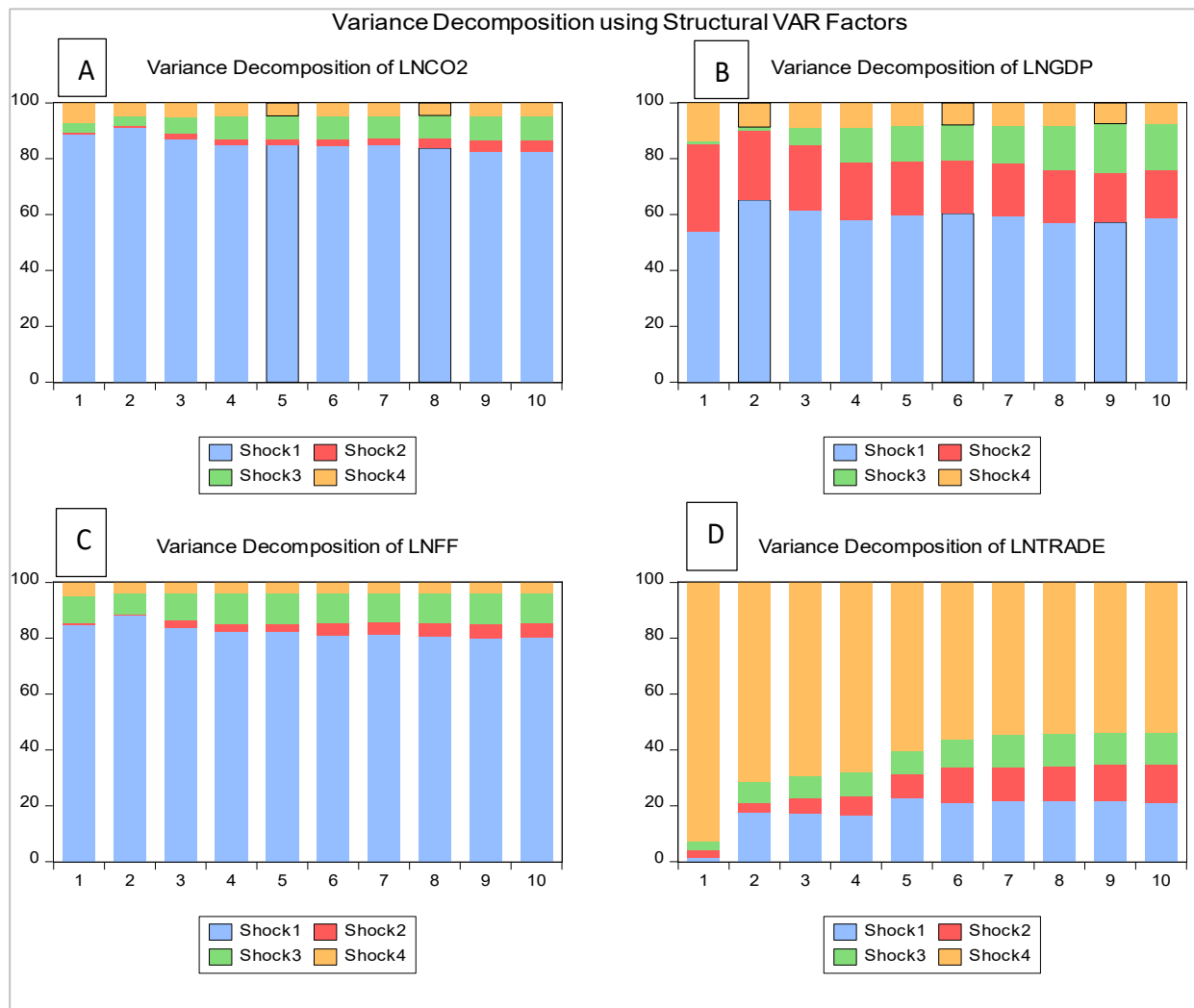
Figure 5.15 Forecast Error Variance Decomposition in the USA. Source: Computed by the authors.
