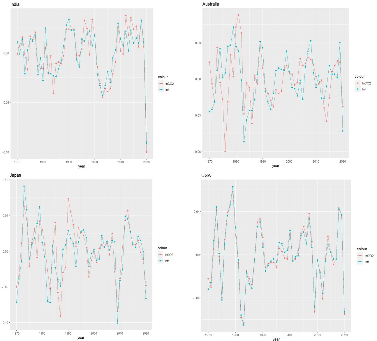
Figure 5.7 Co-Movement of CO 2 emissions and fossil fuel consumption cycles.
