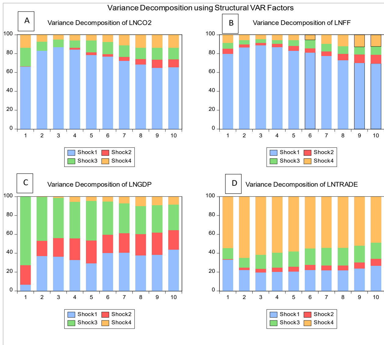
Figure 5.14 Forecast Error Variance Decomposition in India. Source: Computed by the authors.
