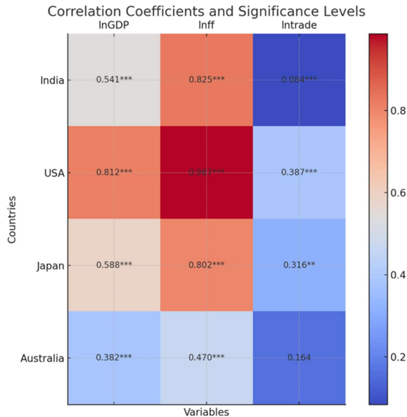
Figure 5.9 Pearson correlation of GDP, fossil fuel, and Trade with CO 2 emissions.
