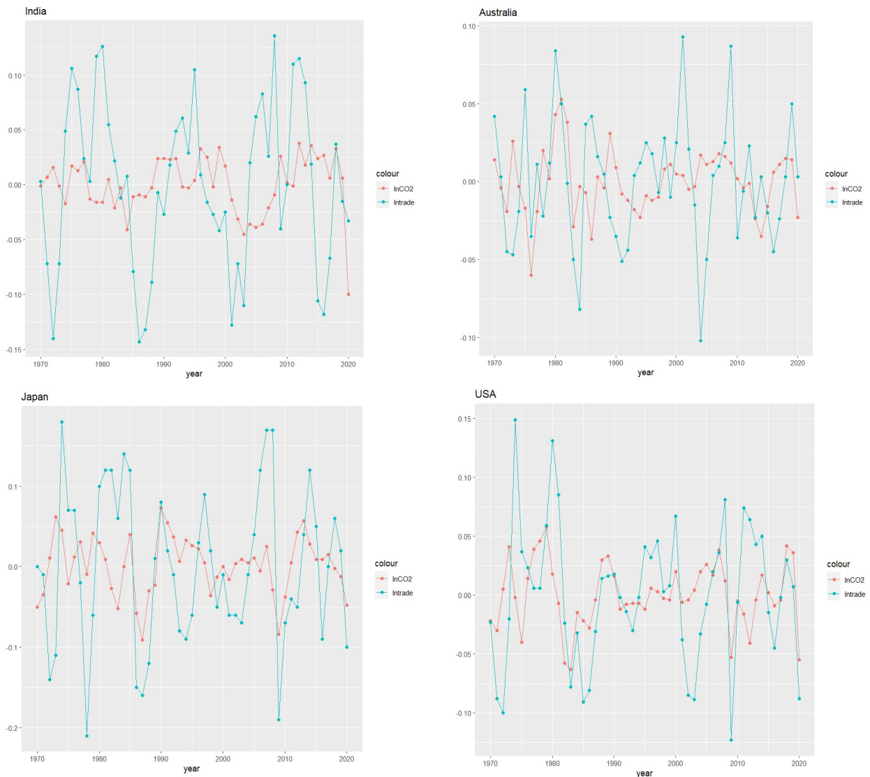
Figure 5.8 Co-Movement of CO 2 emissions and trade cycles.
