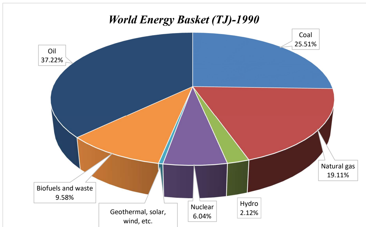
Figure 1.1 Share of world energy in 1990.
