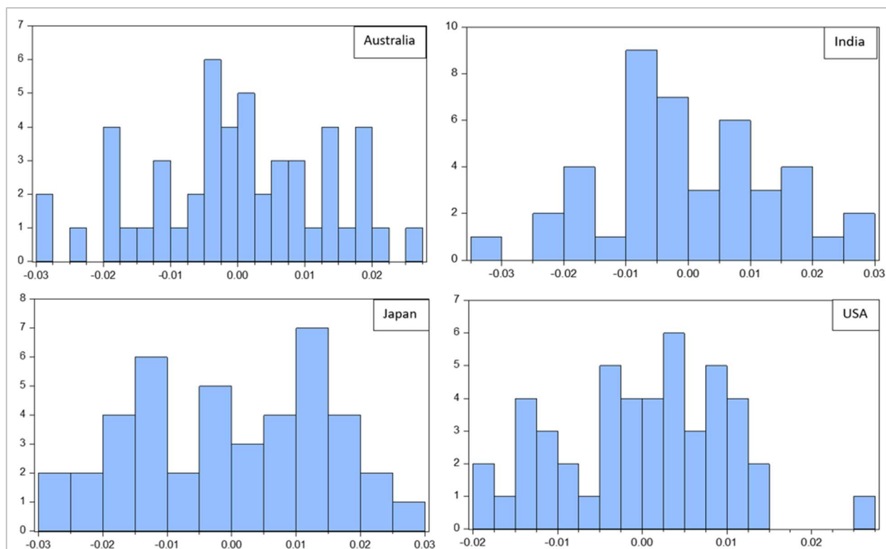
Figure 5.23 Normality test results for QUAD nations. Source: Computed by the authors.
