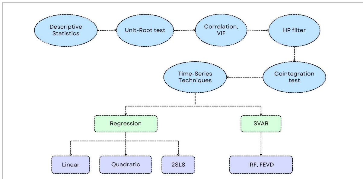
Figure 4.3 Methodological Framework
