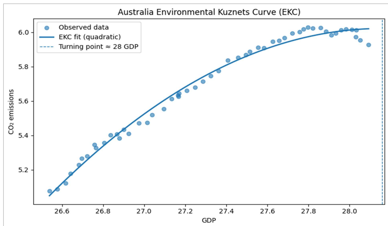
Figure 5.20 EKC for Australia. Source: Computed by the authors.
