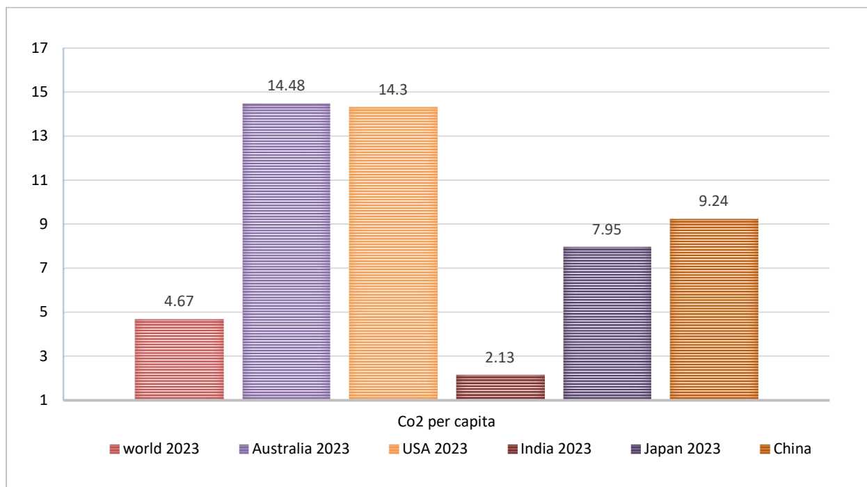
Figure 5.1 CO 2 emissions per capita-2023.
