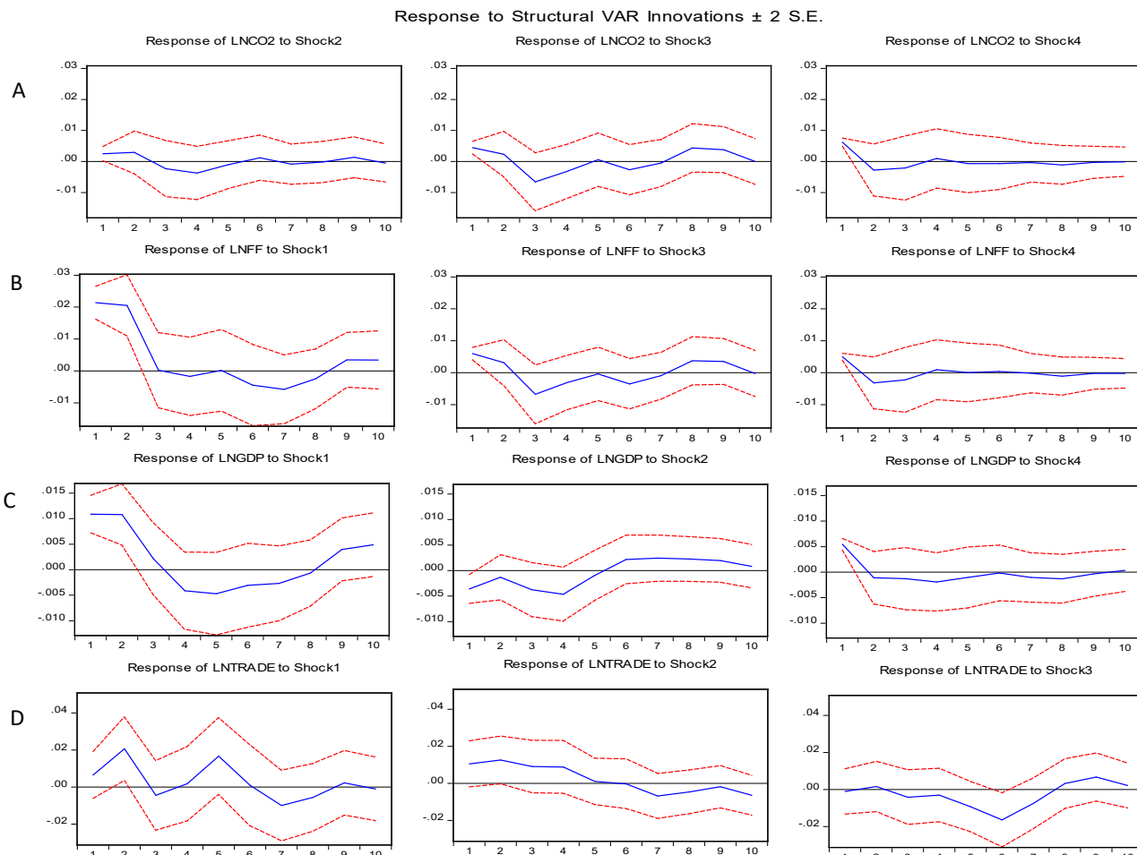
Figure 5.11 Structural Impulse Response Function with one innovation shock in CO 2 emissions for the USA.
