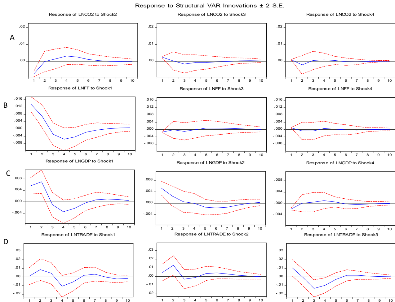
Figure 5.12 Structural Impulse Response Function with one innovation shock in CO 2 emissions for Australia.
