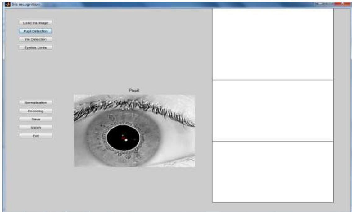
Figure 5.34 : Pupil detection
