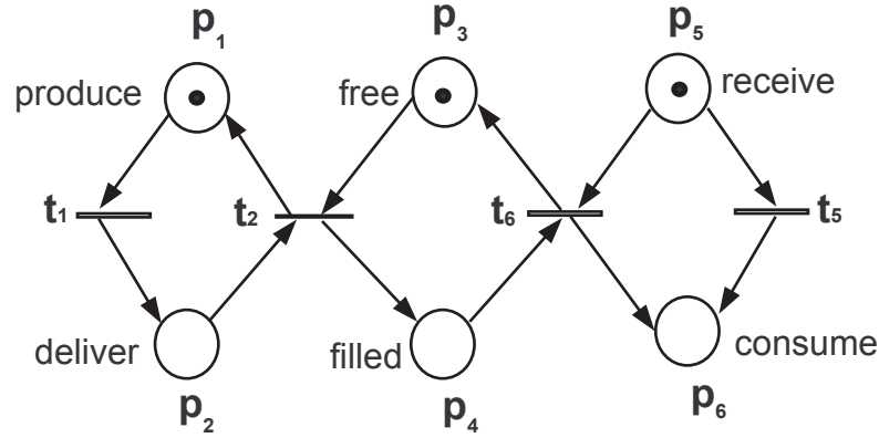
Figure 6.3: Reduced Petri net for producer/consumer problem
