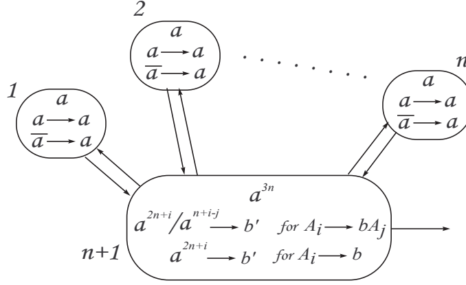
Figure 3.2: SN PA system generating binary regular languages
