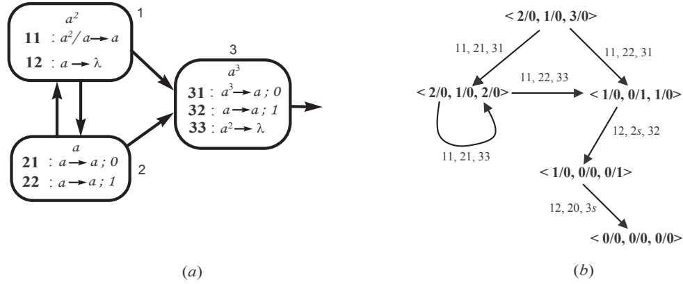
Figure 4.6: (a) An SN P system \Pi_1 (b) Evolution of \Pi_1
