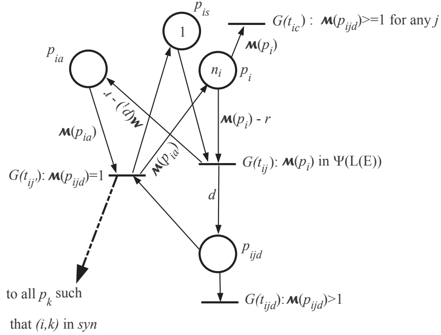
Figure 4.1: Sub net for the rule ij : E/a^r \rightarrow a; d
