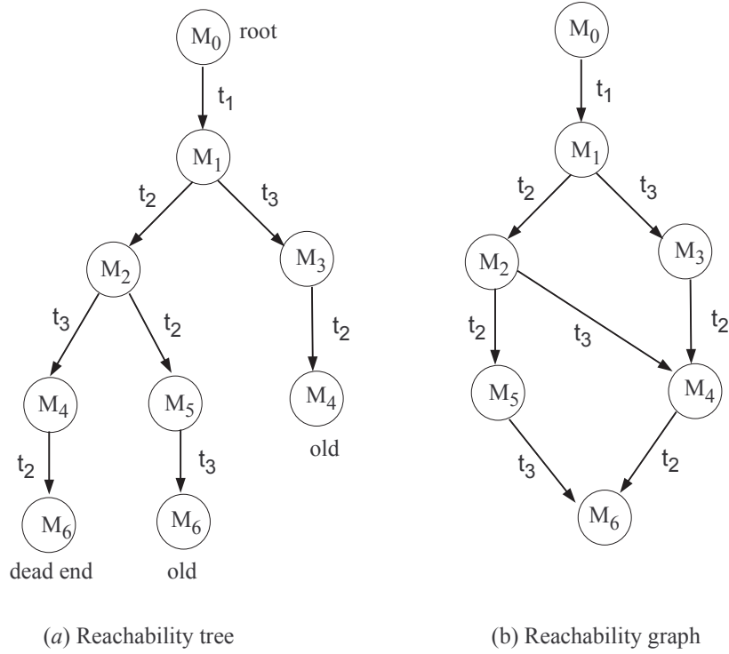
Figure 2.7: Reachability analysis.
