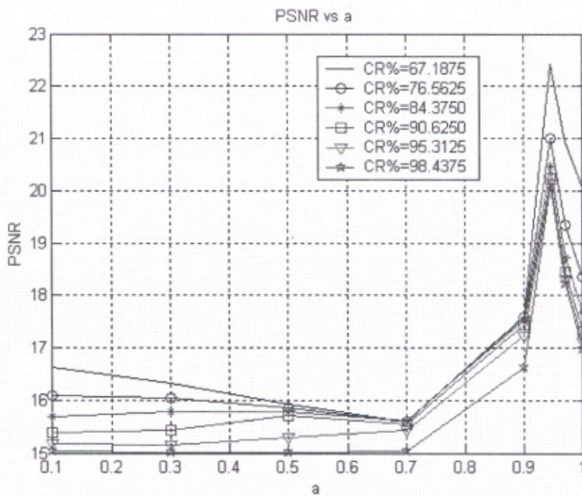
Figure 6.40: PSNR versus 'a' for different values of CR% for Rice image
