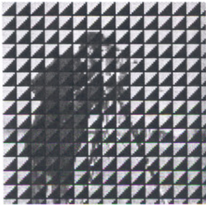
Fig6.16(c) Compressed Cameraman image ( \alpha=.1 , CR%=67.1875, RMSE=52.0143)
