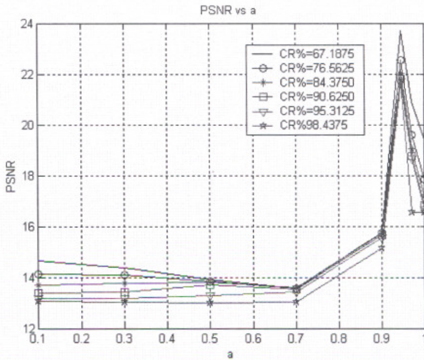
Figure 6.30: PSNR versus 'a' for different values of CR% for Flower image
