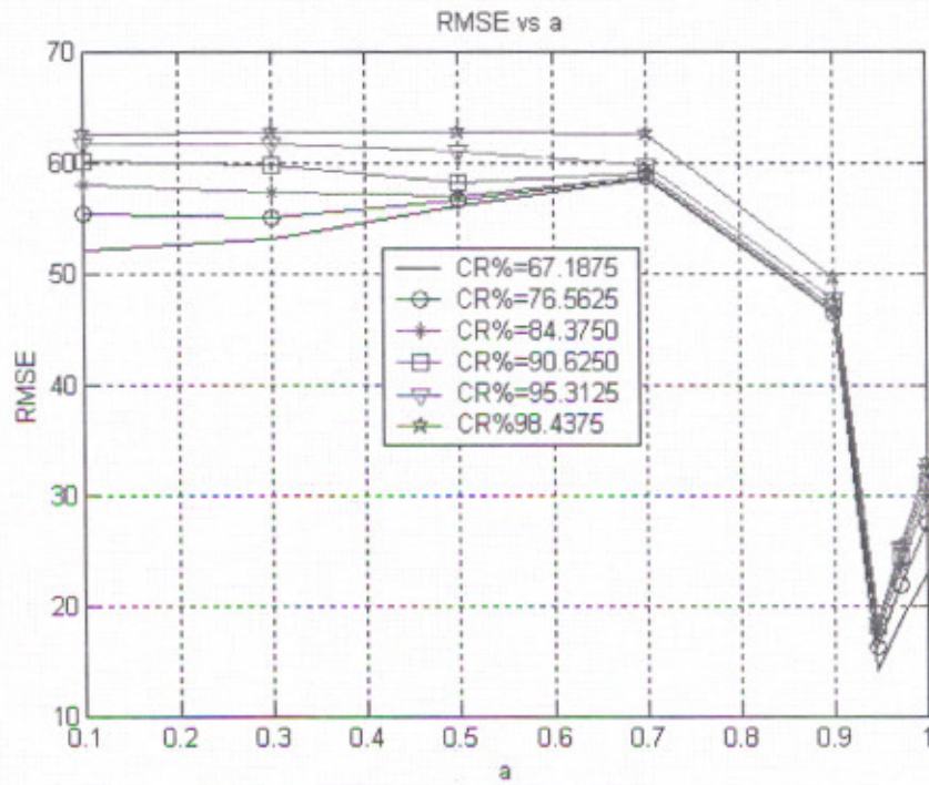
Figure 6.19: RMSE versus 'a' for different values of CR% for Cameraman image
