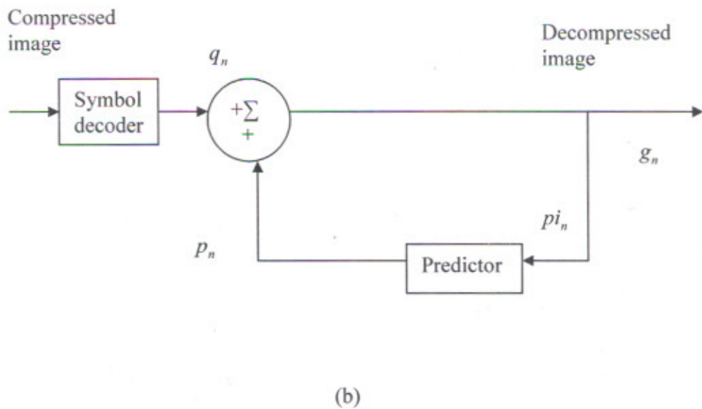
Figure 3.6: A lossy predictive coding model: (a) Encoder, (b) Decoder
