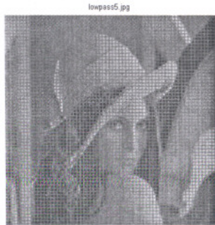
Fig6.4(d)Decompressed Lena image ( \alpha=0.9 , CR%=84.3750, RMSE=33.2890)
