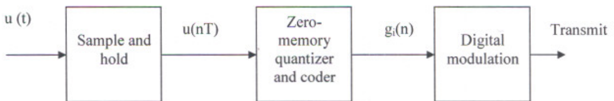
Figure 3.1: Block diagram of PCM
