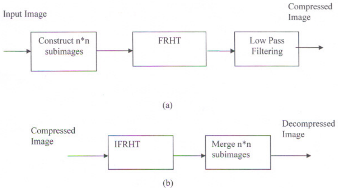
Figure 5.1: FRHT image compression model, (a): Encoder, (b): Decoder
