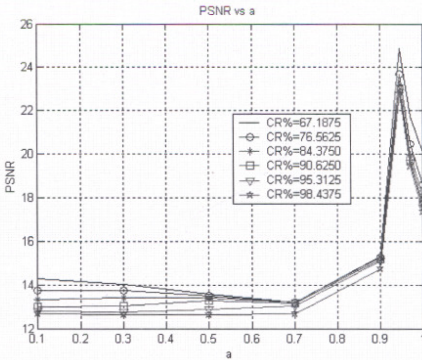
Figure 6.50: PSNR versus 'a' for different values of CR% for Barbara image
