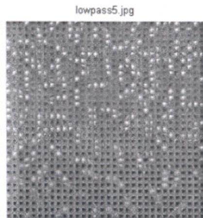
Fig6.35(d)Decompressed Rice image ( a=.5 , CR\%=84.3750 , RMSE=41.3816 )
