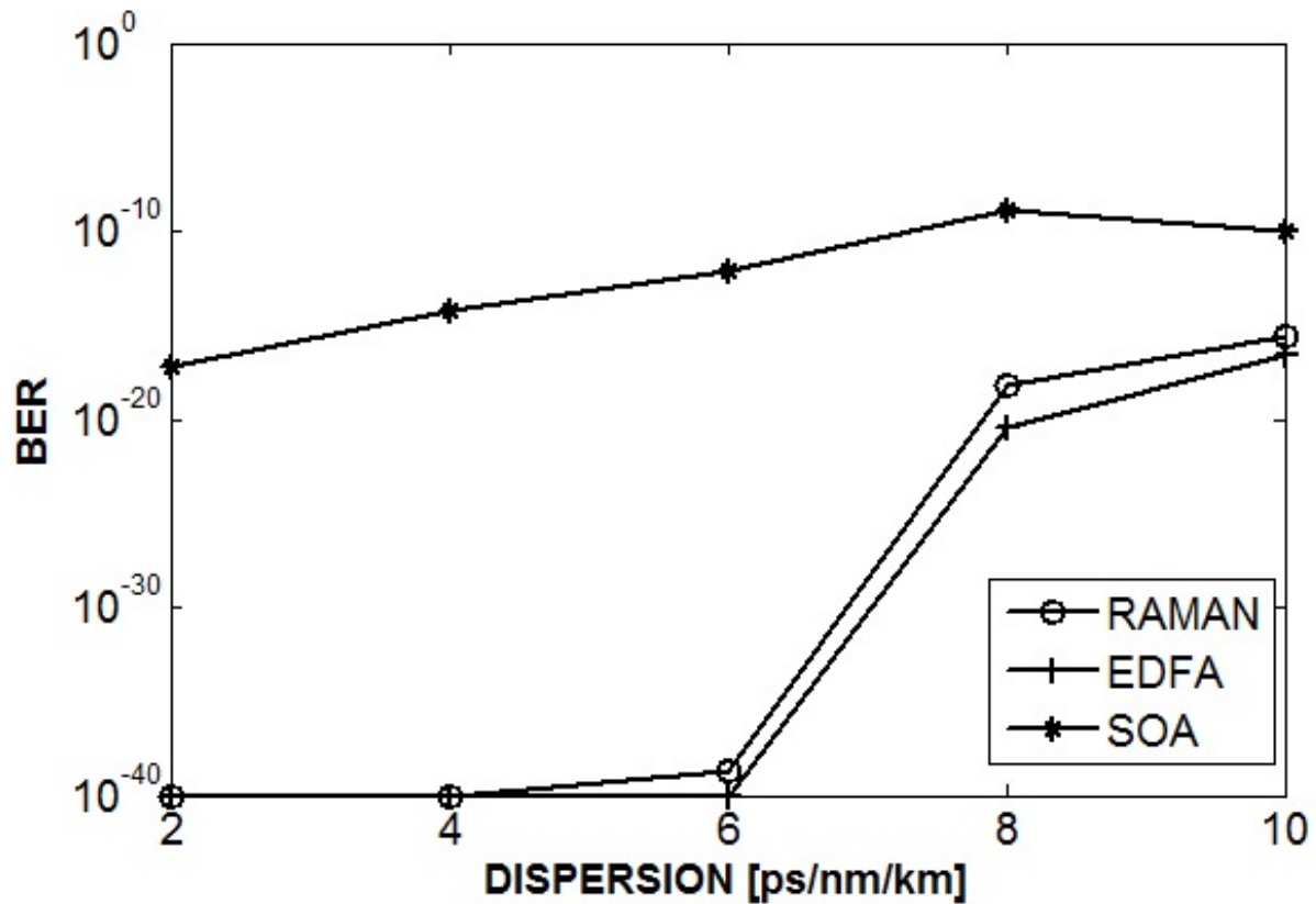
Figure 3.20: BER vs. Dispersion for 16 channels in the presence of nonlinearities
