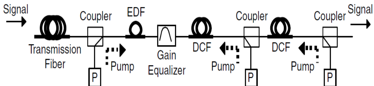
Figure 1.17: Type-4 with large discrete Raman gain
