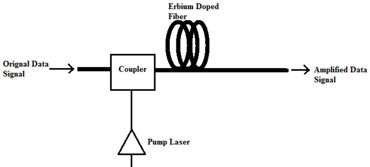
Figure 1.7: Erbium Doped Fiber Amplifier
