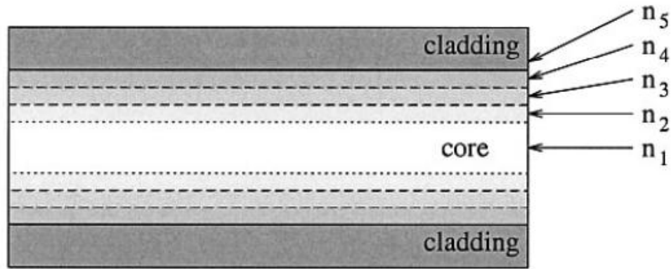
Figure 1.3: Graded-index fiber [6].
