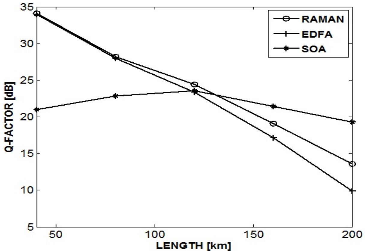
Figure 3.11: Q- factor vs. Length for 32 channels in the absence of nonlinearities
