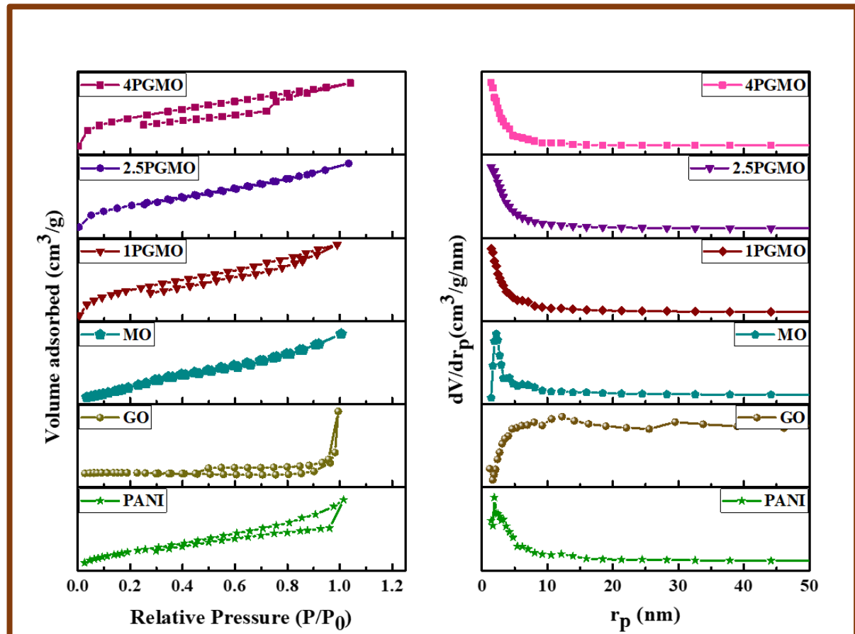
Fig 3.4: (a) Adsorption-Desorption curves of PANI, GO, MoO 3 ,1PGMO,2.5PGMO,4PGMO (b) BJH plot of PANI, GO, MoO 3 ,1PGMO,2.5PGMO,4PGMO.
