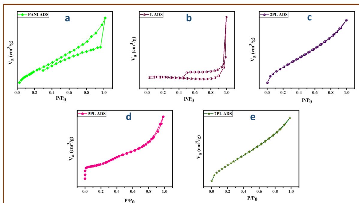
Fig 5.7: (a), (b), (c), (d), and (e) adsorption-desorption curves of PANI, L, 2PL, 5PL, and 7PL respectively.
