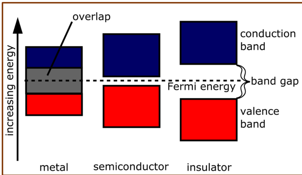
Fig 1.1: Comparative energy band structures of metals, semiconductors, and insulators.
