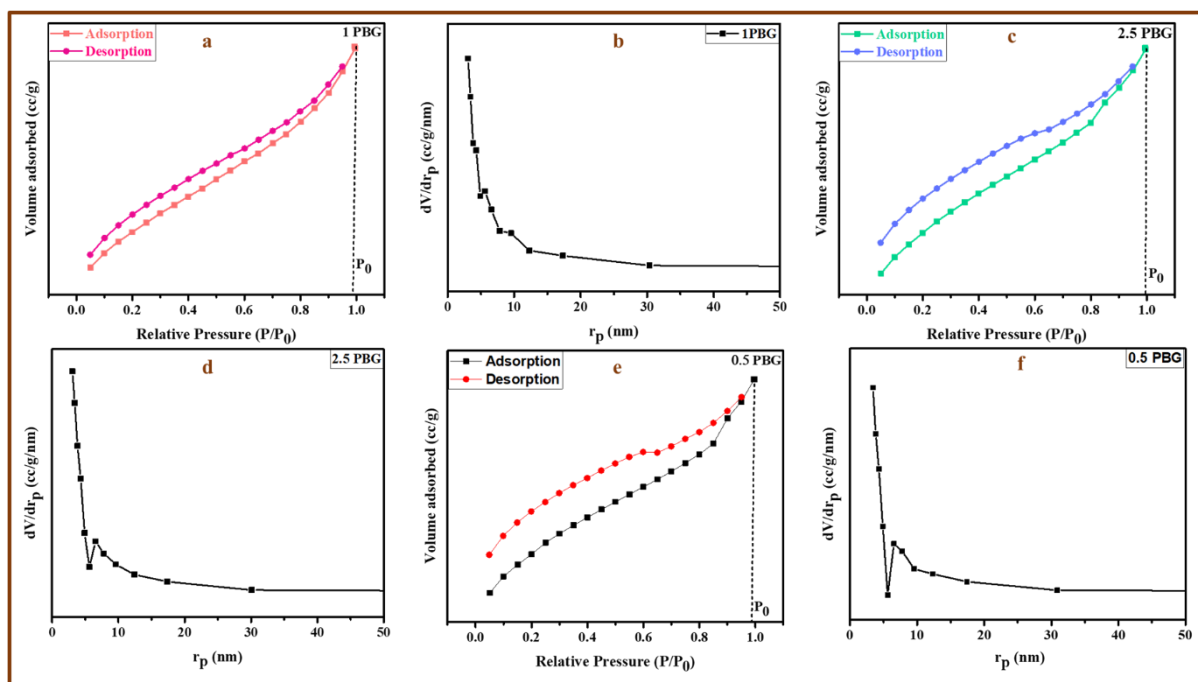
Fig 2.4: (a), (c), and (e) are adsorption-desorption curves 1PBG, 2.5 PBG, and 0.5 PBG
