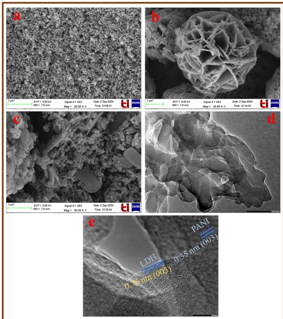
Fig 5.5: FESEM image of (a) PANI, (b) LDH, (c) 5PL, and HRTEM images (d-e) of 5PL.
