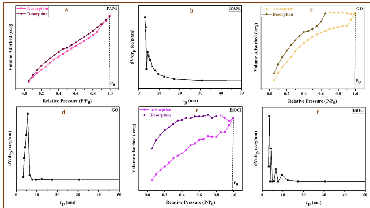
Fig 2.3: (a), (c), and (e) are adsorption-desorption curves of PANI, GO, and BiOCl respectively, whereas (b), (d), and (f) are BJH plots of PANI, GO, and BiOCl respectively.
