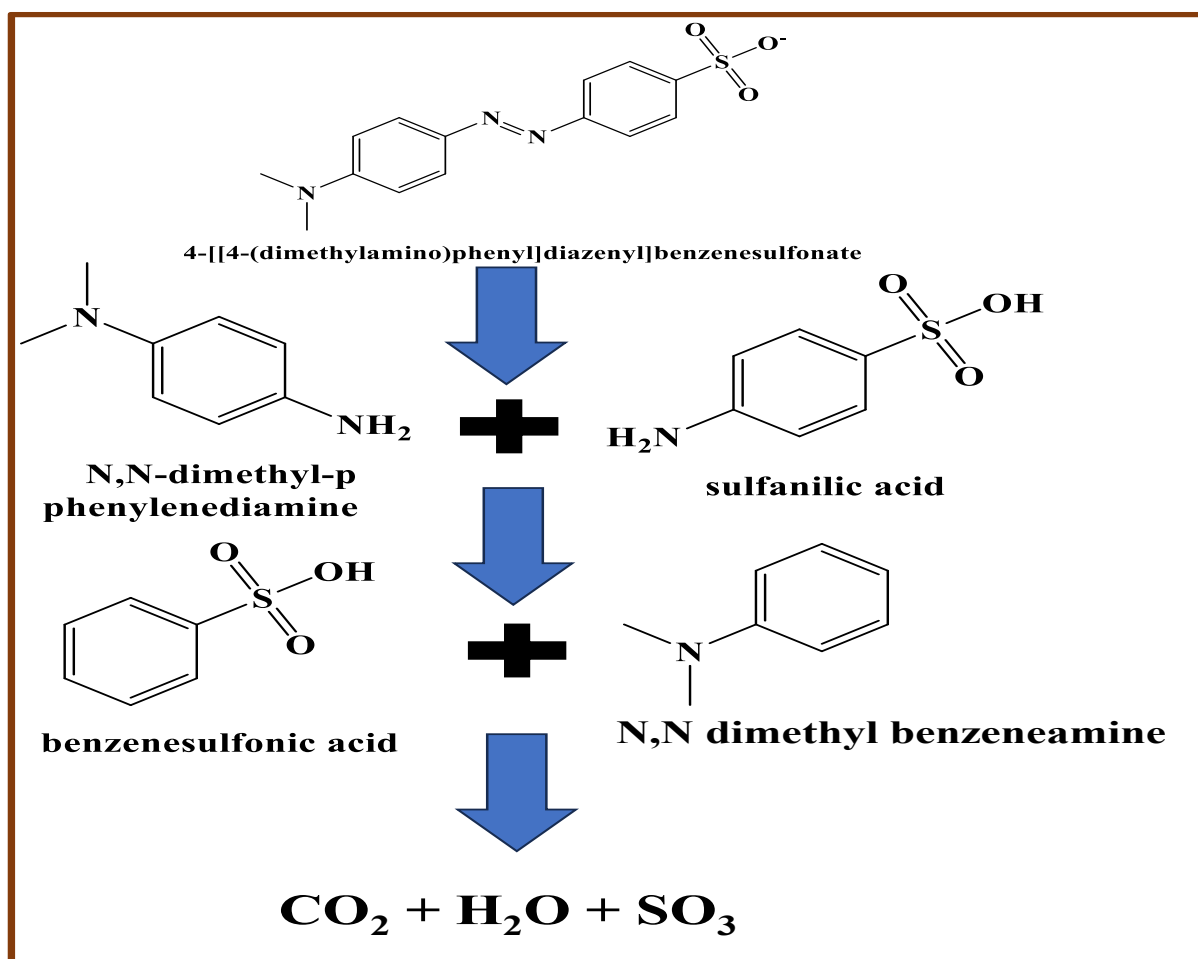
Fig 3.12: Potential pathway for photocatalytic degradation of methyl orange using the 2.5PGMO photocatalyst.
