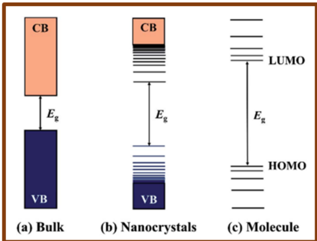
Fig 1.2: Energy Level Diagrams of Bulk, Nanocrystal, and Molecular Systems.
