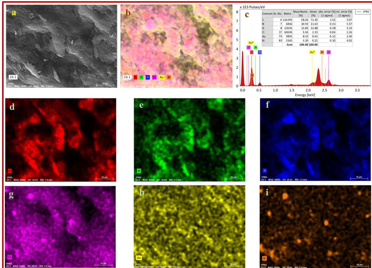
Fig 2.2: (a) FESEM image of 1PBG, (c) EDS spectrum of 1PBG and (b, d-e) is the elemental mapping of its constituents.
