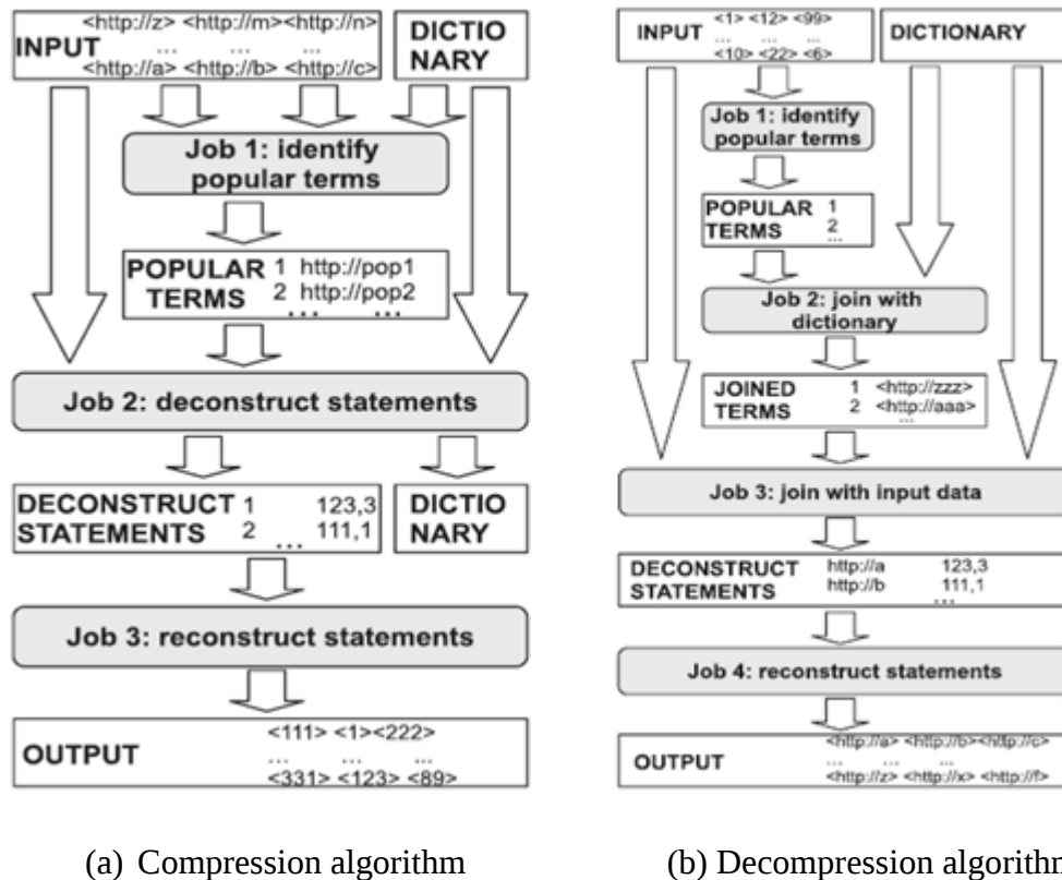
Figure 2.1: Compression and decompression of RDF[26]
