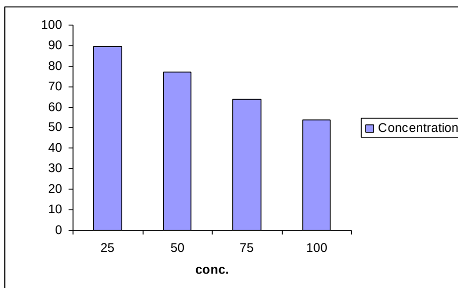
Fig-4.8 Effect of concentration on photocatalytic degradation of 2-nitroaniline [pH] =2, [wavelength] = 282nm, [ \text{TiO}_2 ] =4g/L, [Time] =6hrs
