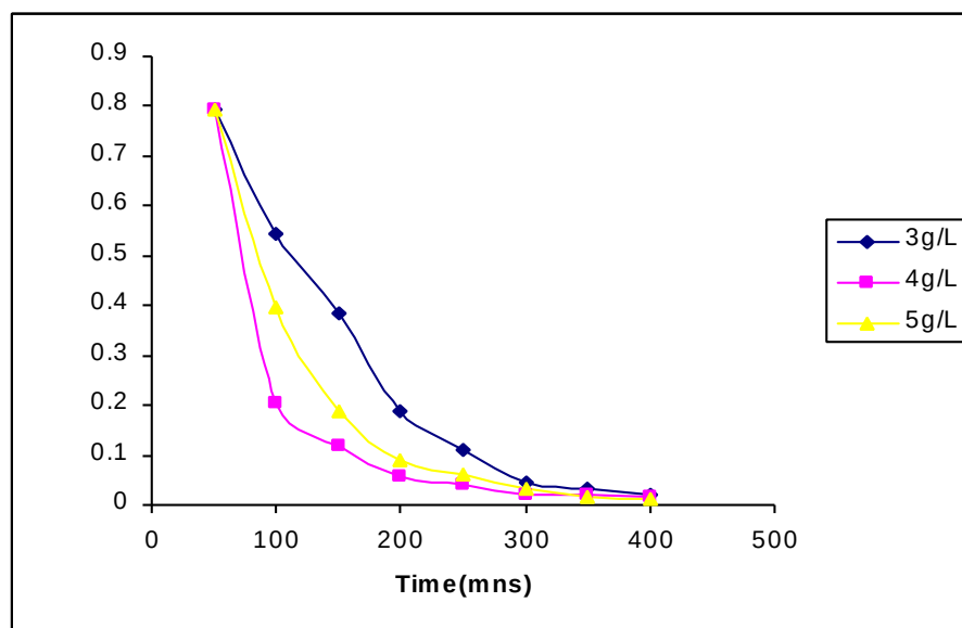
Fig-4.5 Effect of catalyst dose on decolourisation of 2-nitroaniline compound
