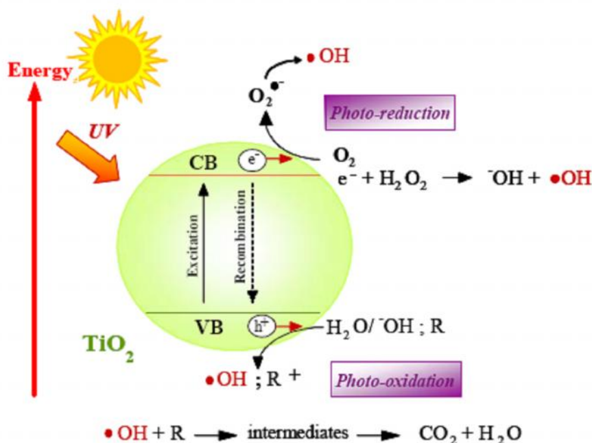
Fig-1.3 Irradiated \text{TiO}_2 semi-conductor particle
