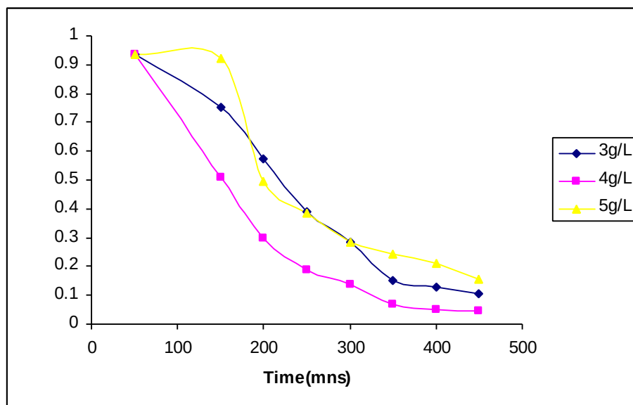
Fig-4.4 Effect of catalyst dose on photocatalytic degradation of 2-nitroaniline
