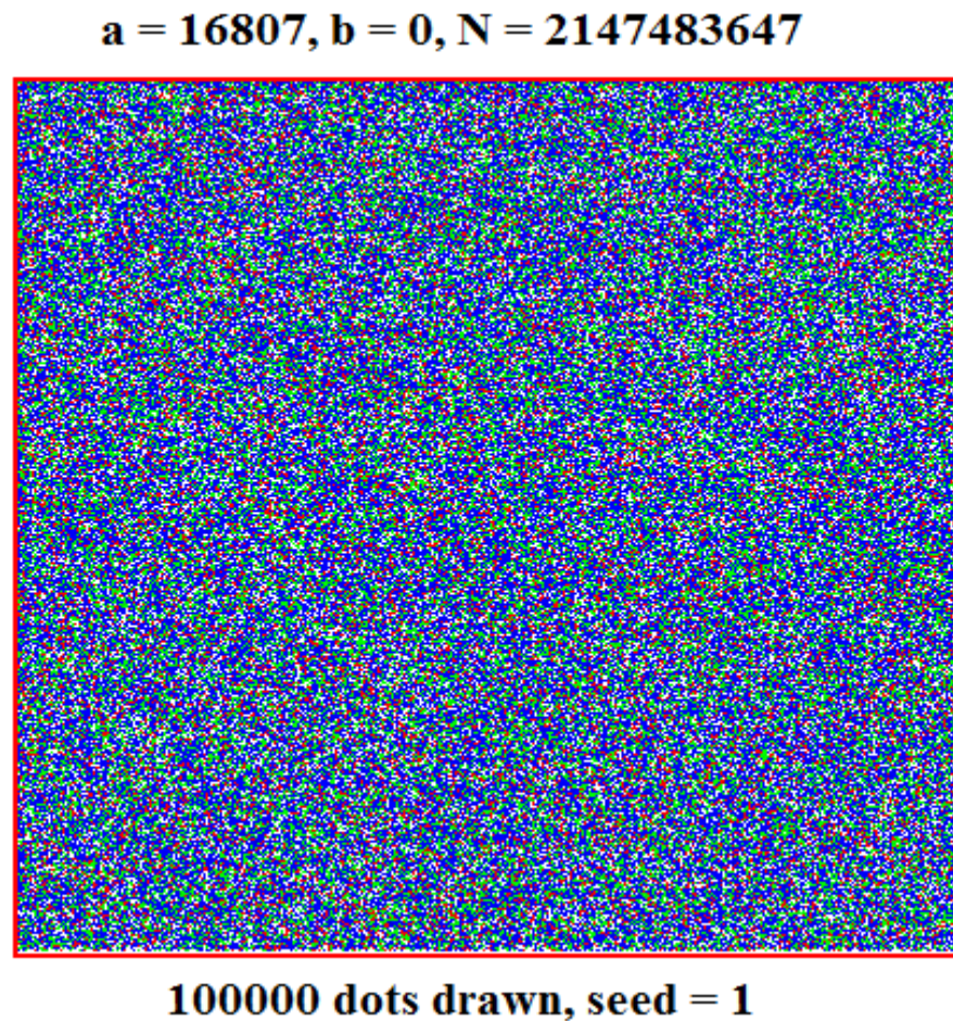
Figure 1.2: Generating 100000 random dots [18]
