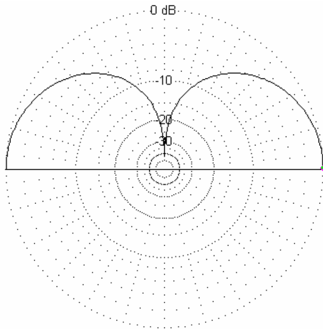
Figure3.9(c): Elevation plot of total field for 5.1c.m. long Koch fractal monopole with two iteration
