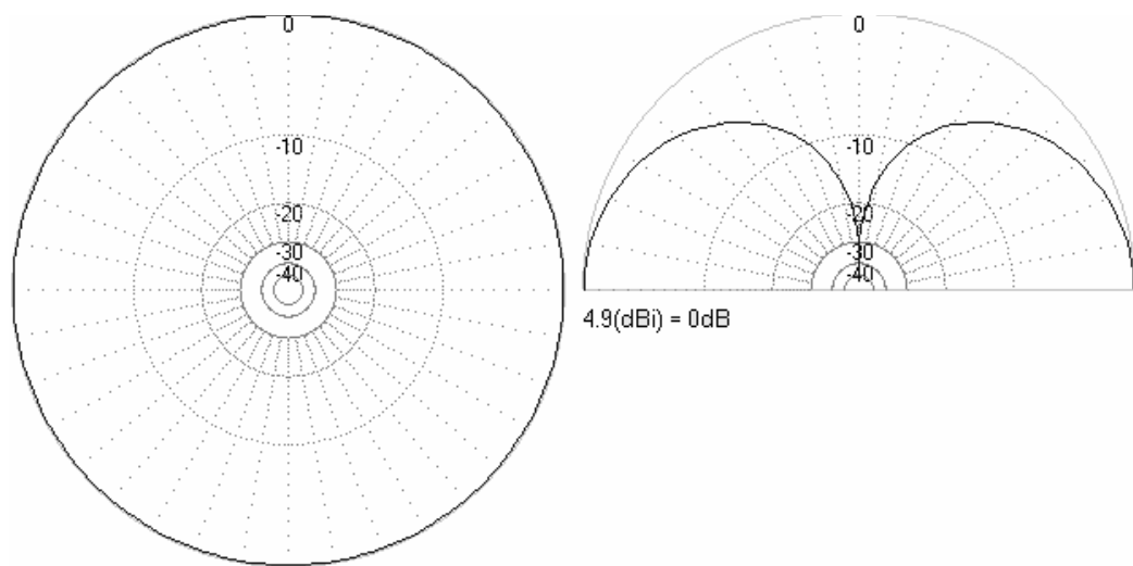
Figure 4.2(d): Azimuthal and elevation plot of Radiation Pattern
