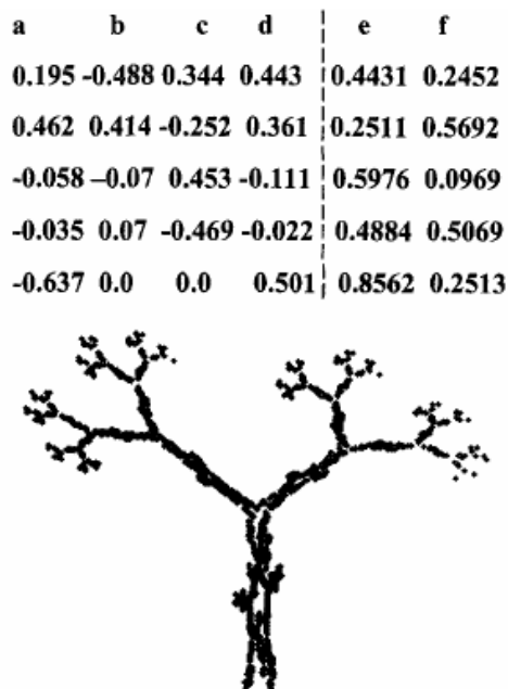
Figure 2.8: The iterated function system code for a fractal tree[16].
