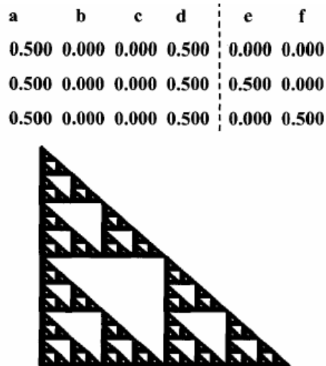
Figure 2.7: The iterated function system code for a Sierpinski gasket[16].
