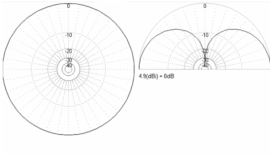
Figure 5.6(d): Azimuthal and elevation plot of Radiation Pattern
