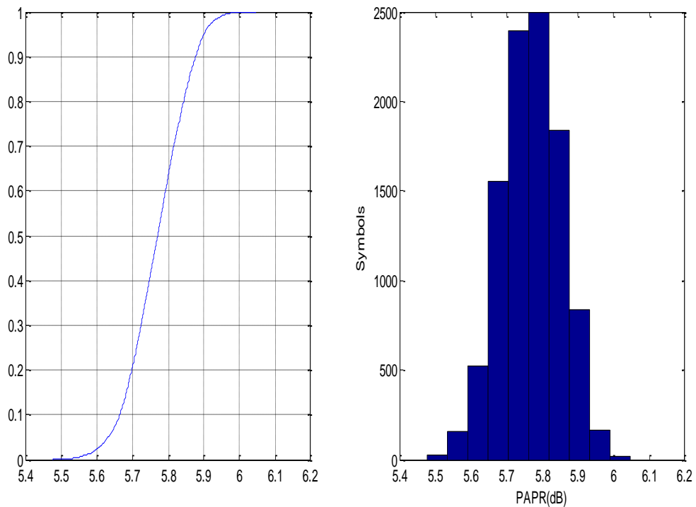
Fig. 7.22: PAPR for GMSK after applying SLM with U=30 (a) CCDF (b) Histogram
