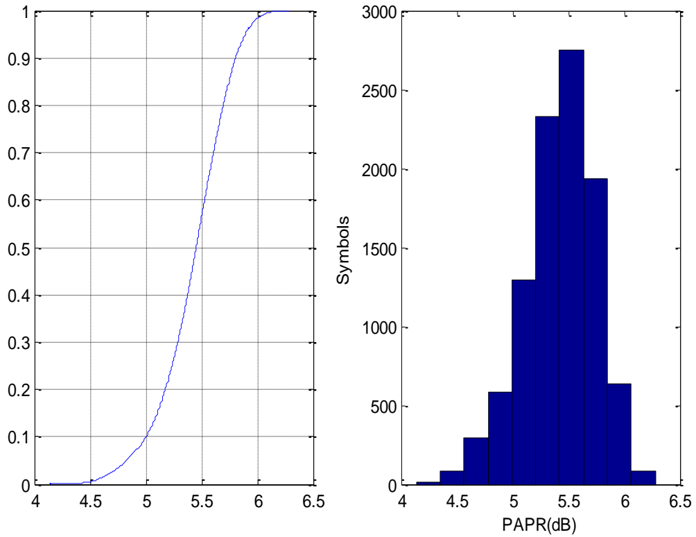
Fig. 7.16: PAPR for 64PSK after applying SLM with U=30 (a) CCDF (b) Histogram
