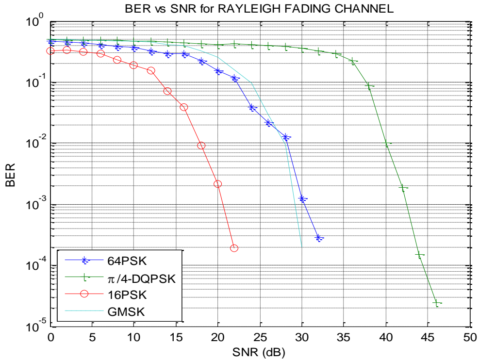
Fig. 7.5: BER performance for different modulation schemes over Rayleigh fading channel
