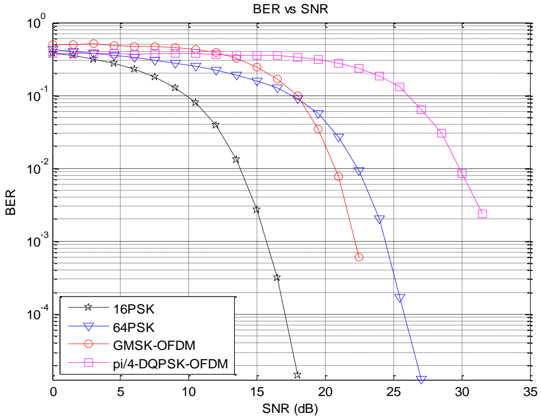
Fig. 7.4: BER performance for different modulation schemes over AWGN channel
