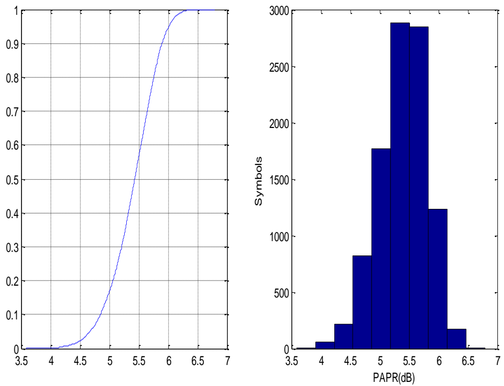
Fig. 7.15: PAPR for 64PSK after applying SLM with U=20 (a) CCDF (b) Histogram
