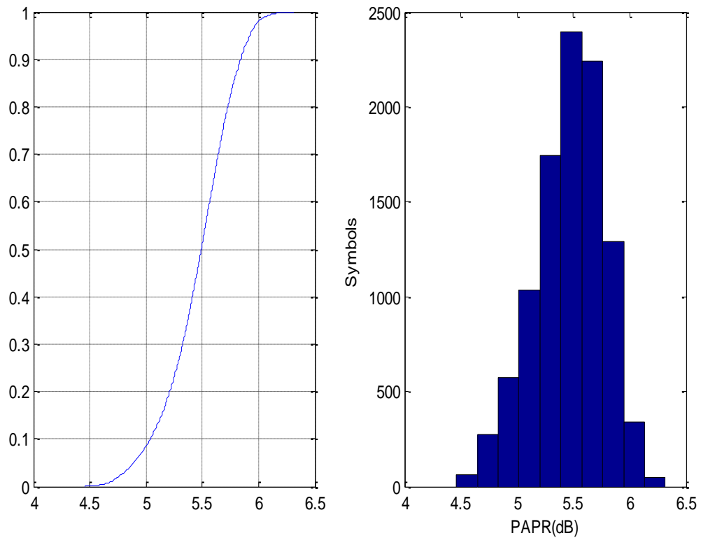
Fig. 7.19: PAPR for \pi/4 –DQPSK after applying SLM with U=30 (a) CCDF (b) Histogram
