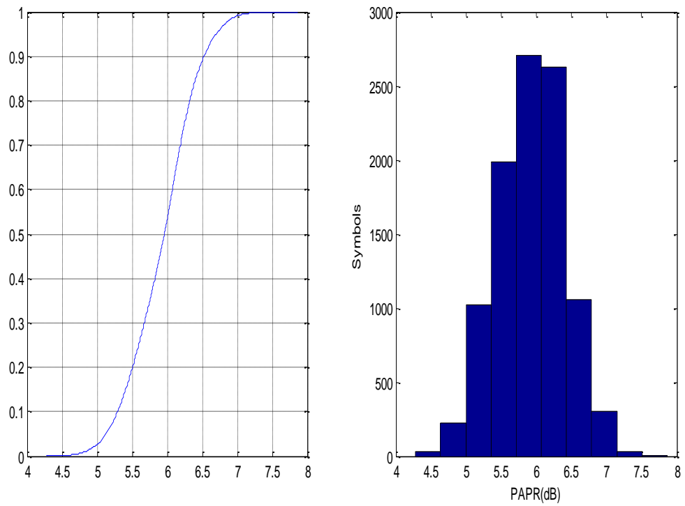
Fig. 7.20: PAPR for GMSK after applying SLM with U=10 (a)CCDF (b) Histogram
