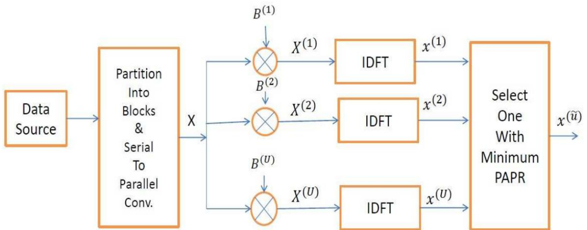
Fig. 4.2: Block Diagram of SLM[9]
