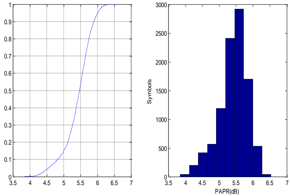
Fig. 7.18: PAPR for \pi/4 -DQPSK after applying SLM with U=20 (a) CCDF (b) Histogram
