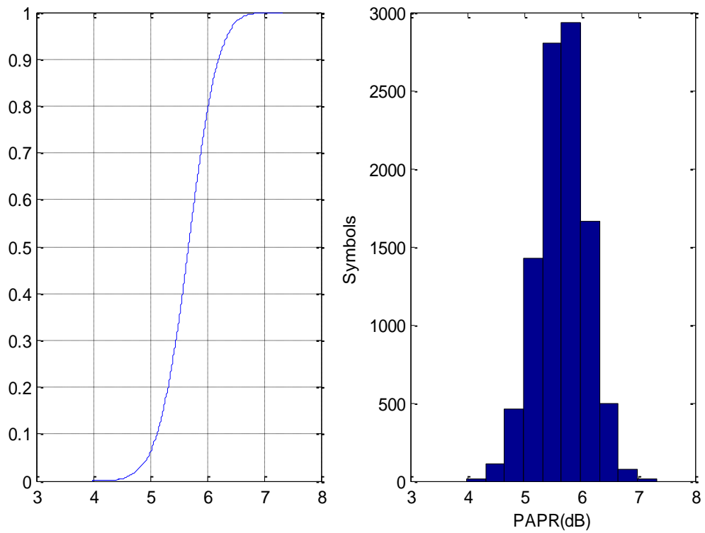
Fig. 7.14: PAPR for 64PSK after applying SLM with U=10 (a) CCDF (b) Histogram
