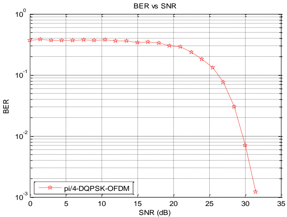
Fig. 7.3: BER performance of \pi/4 –DQPSK over AWGN channel
