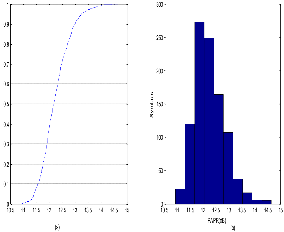
Fig. 7.10: PAPR for GMSK (a) CCDF Function (b) Histogram
