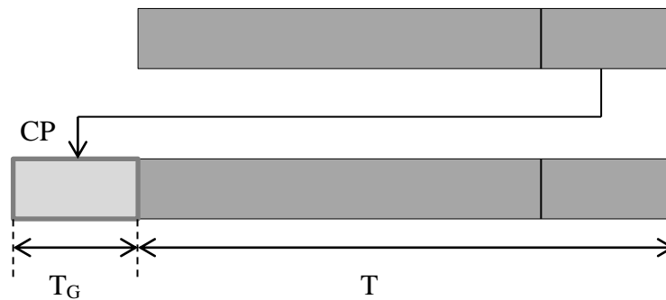
Fig. 3.3 Generate Cyclic Prefix
