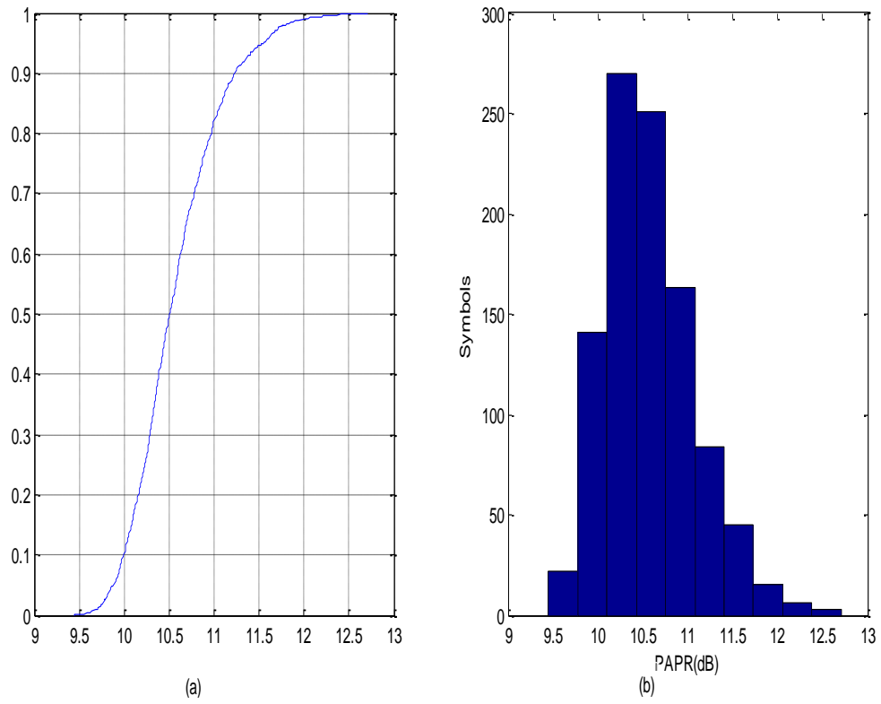
Fig. 7.8: PAPR for 64PSK (a) CCDF Function (b) Histogram
