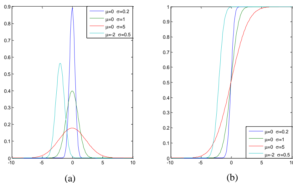
Fig. 6.7: Gaussian distribution (a) PDF (b) CDF
