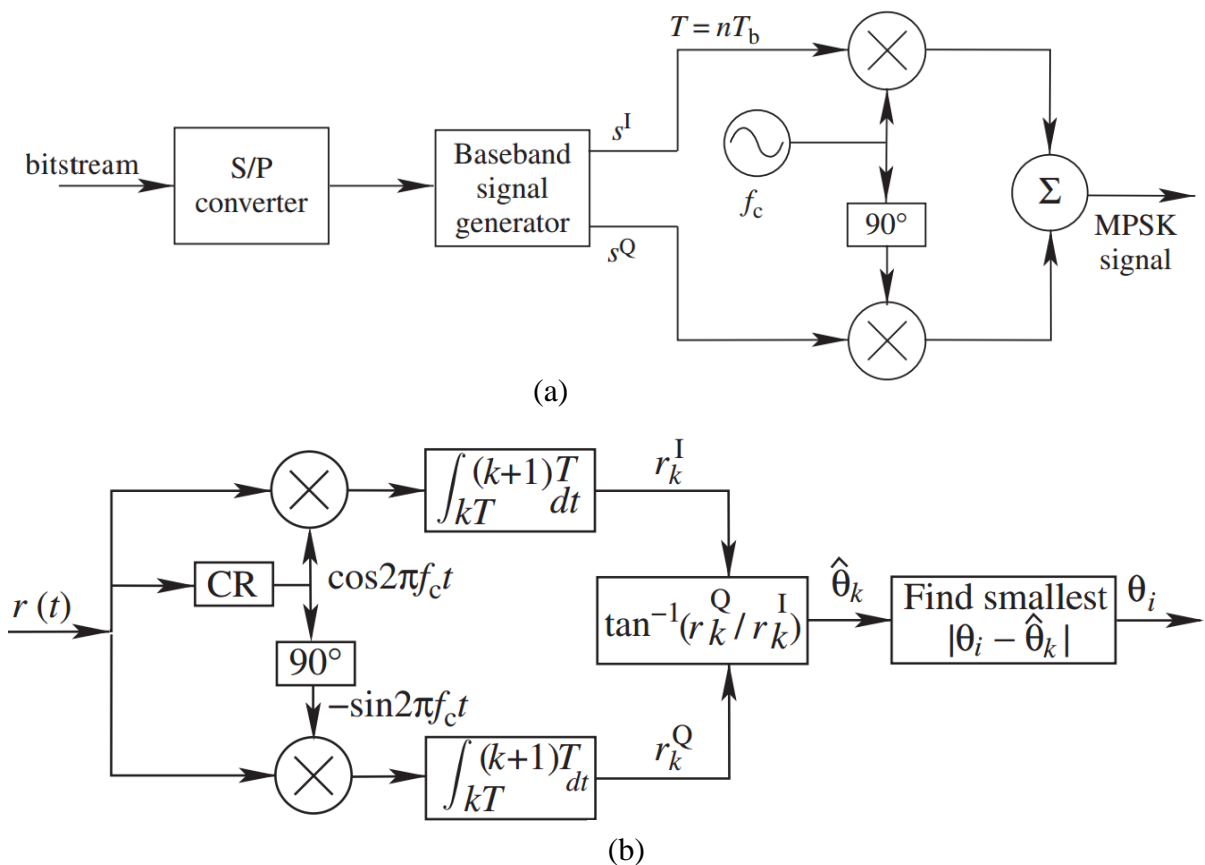
Fig. 5.2: MPSK (a) modulator (b) Coherent MPSK demodulator. CR denotes coherent reference. [49]
