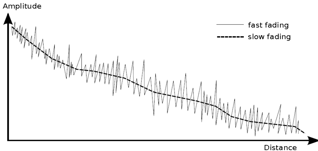
Fig. 6.2 Large scale& small scale fading [4]
