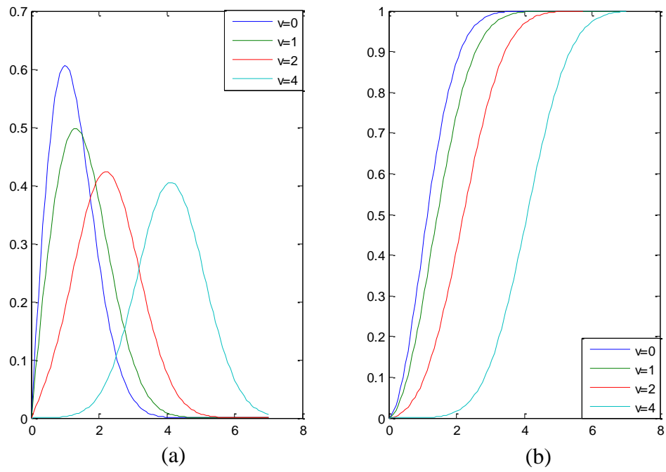
Fig. 6.9 Rician random variable (a) PDF and (b) CDF for \sigma = 1
