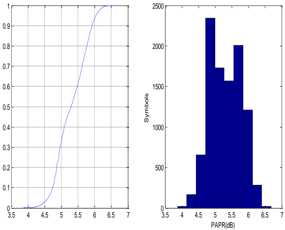
Fig. 7.21: PAPR for GMSK after applying SLM with U=20 (a) CCDF (b) Histogram
