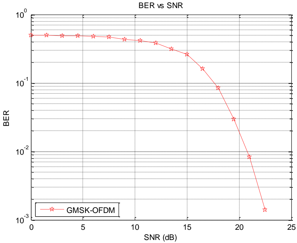
Fig. 7.2: BER performance of GMSK-OFDM over AWGN channel
