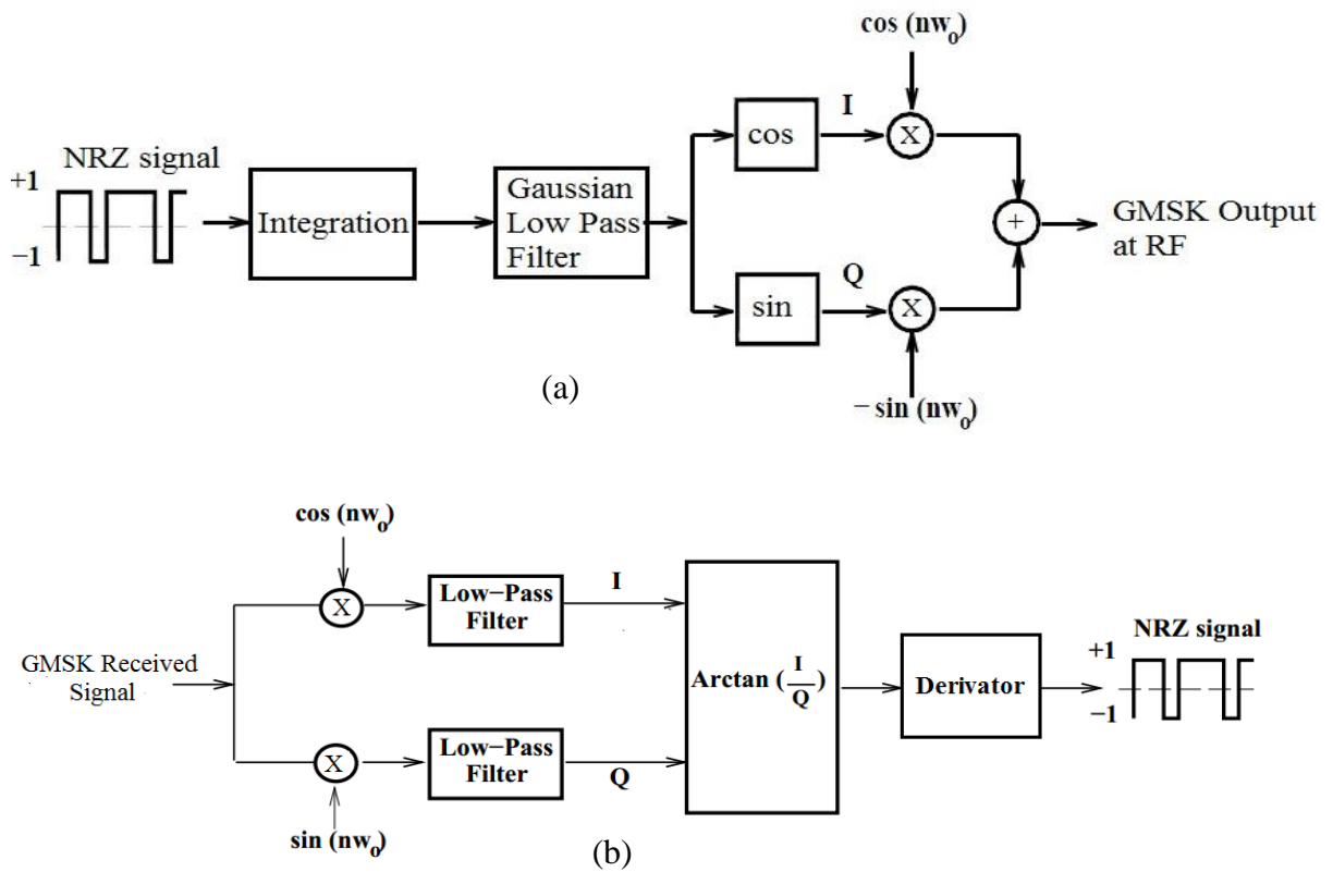
Fig. 5.4: GMSK (a) transmitter (b) receiver
