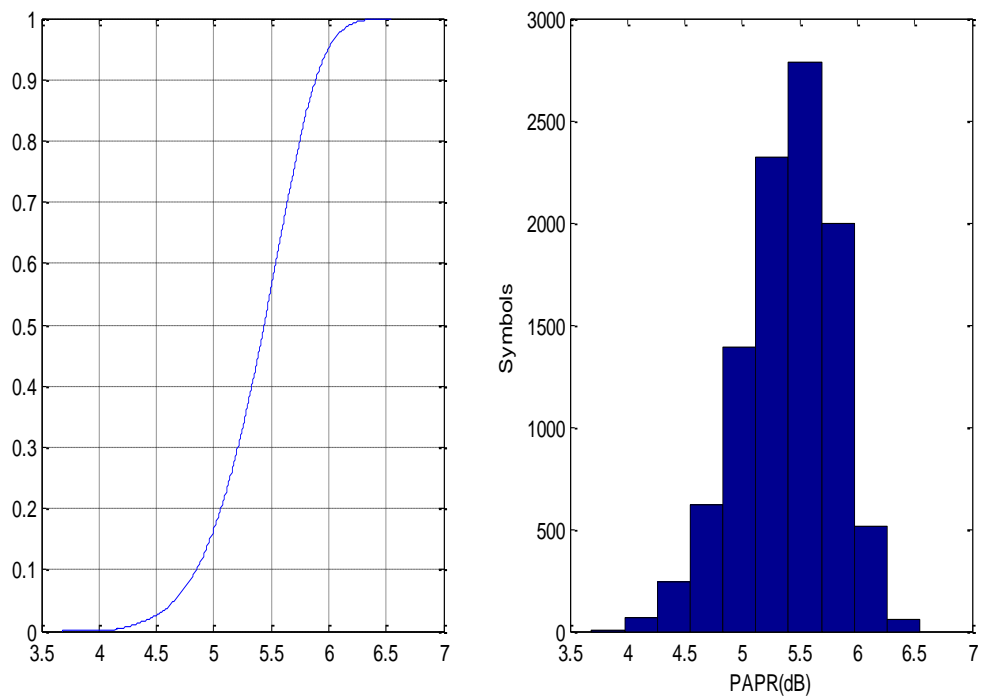
Fig. 7.12: PAPR for 16PSK after applying SLM with U=20 (a) CCDF (b) Histogram
