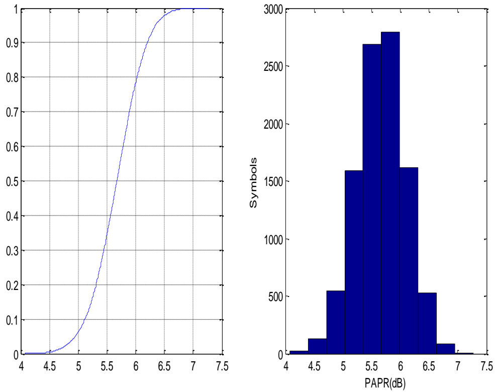
Fig. 7.11: PAPR for 16PSK after applying SLM with U=10 (a) CCDF (b) Histogram
