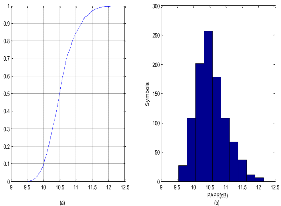
Fig. 7.7: PAPR for 16PSK (a) CCDF Function (b) Histogram
