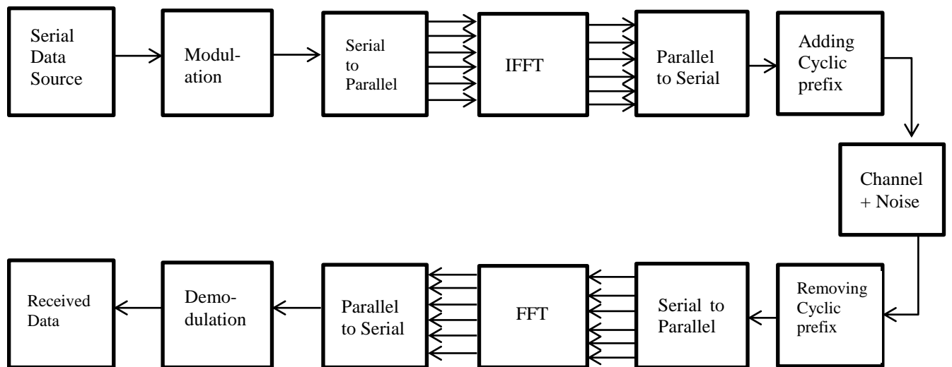
Fig. 3.2: Basic OFDM transceiver
