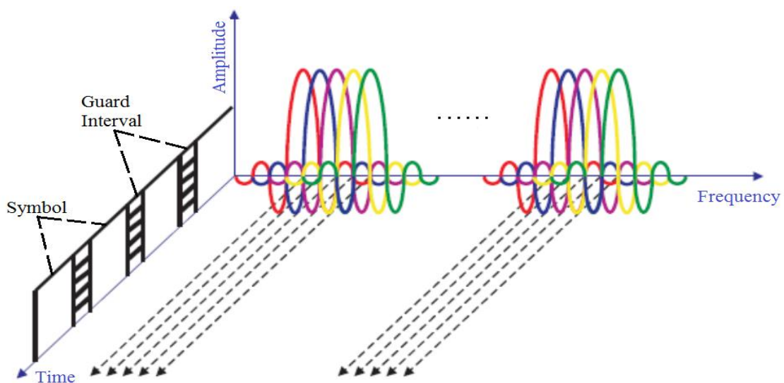
Fig. 3.1: OFDM time/frequency representation [36]
