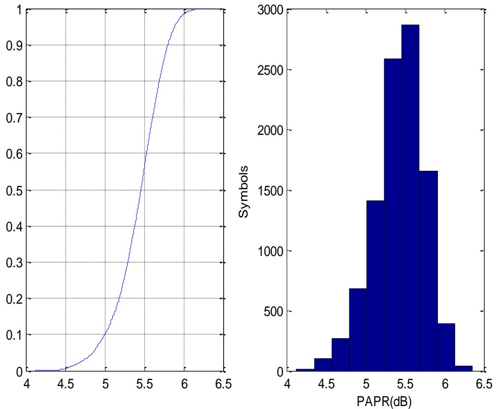
Fig. 7.13: PAPR for 16PSK after applying SLM with U=30 (a) CCDF (b) Histogram
