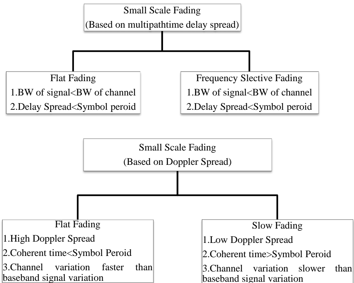
Fig. 6.3: Types of small scale fading [4]
