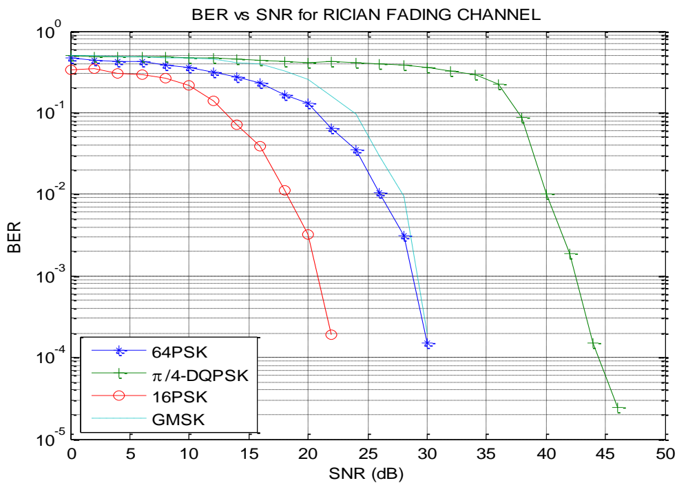
Fig. 7.6: BER performance for different modulation schemes over Rician fading channel
