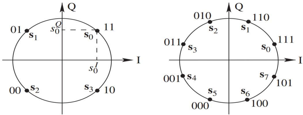
Fig. 5.1: MPSK constellations. (a) QPSK. (b) 8PSK [49]
