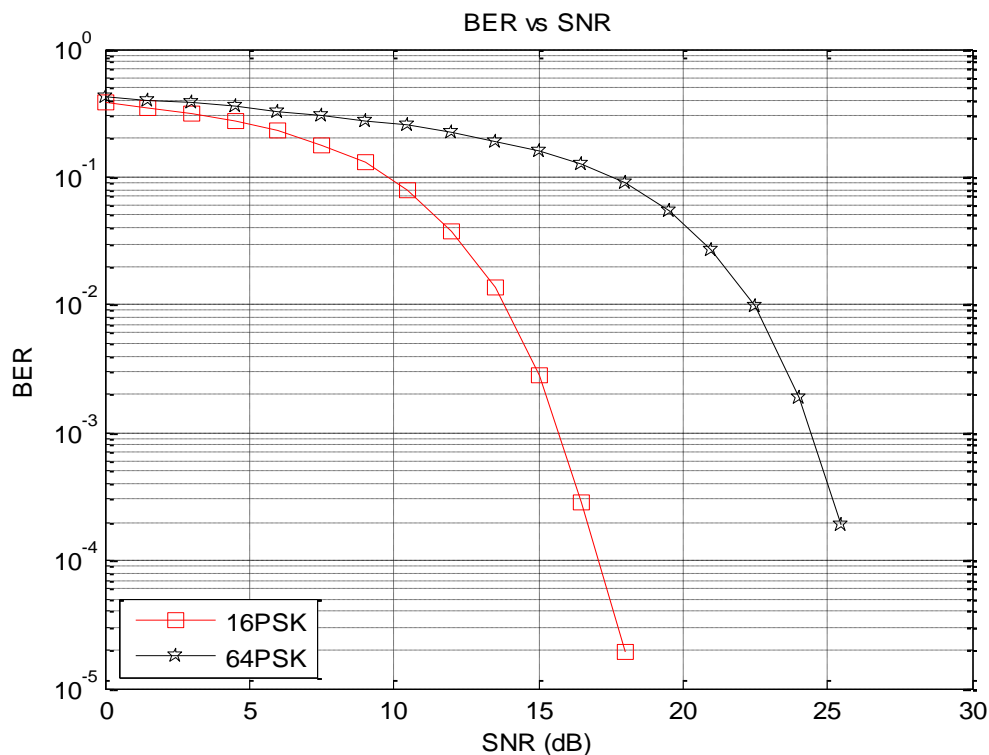
Fig. 7.1: BER performance of 16PSK and 64PSK over AWGN channel
