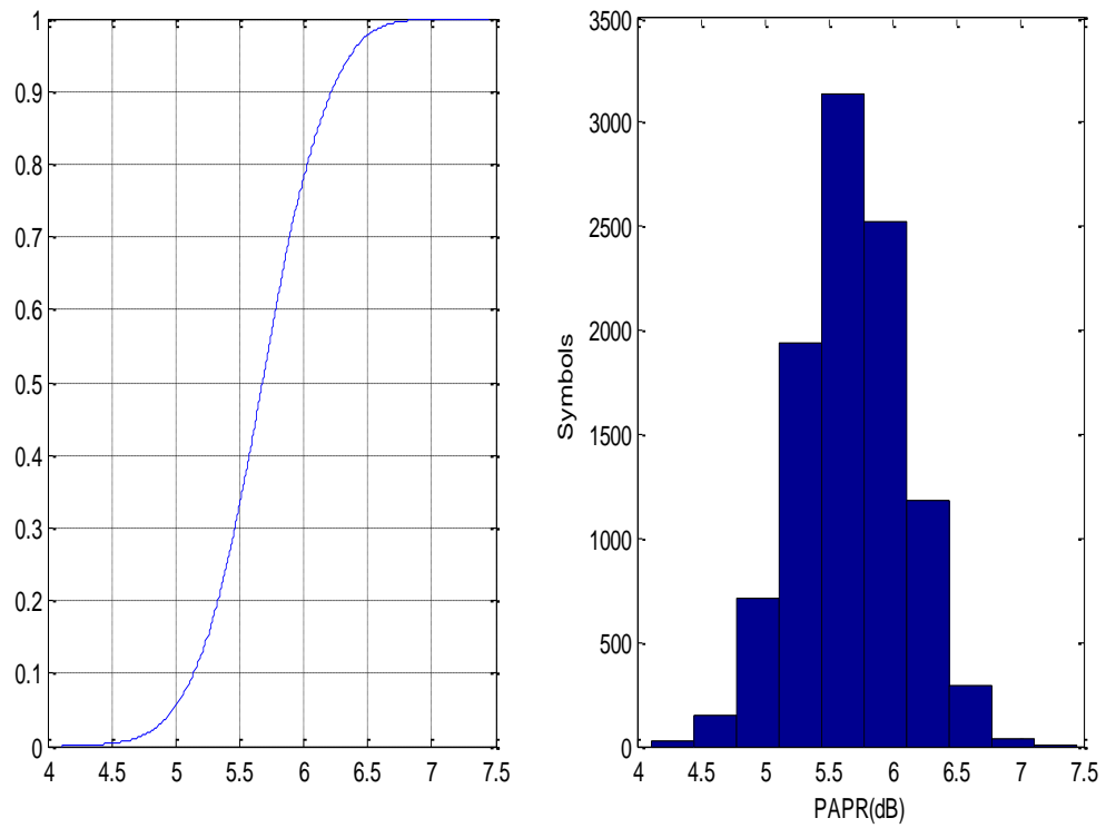
Fig. 7.17: PAPR for \pi/4 -DQPSK after applying SLM with U=10 (a) CCDF (b) Histogram
