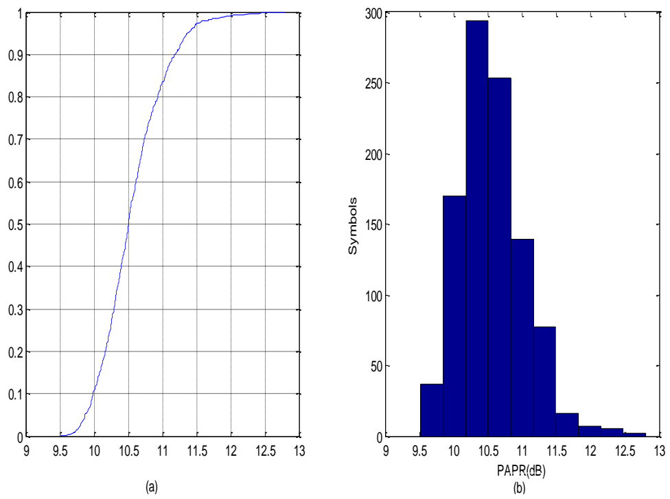
Fig. 7.9: PAPR for \pi/4 -DQPSK (a) CCDF Function (b) Histogram
