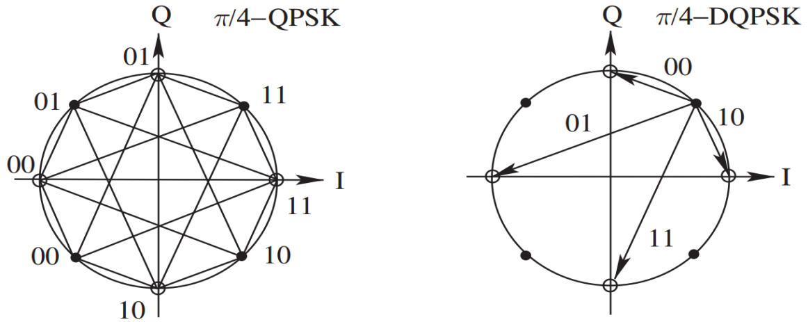
Fig. 5.3: Constellations of \pi/4 - \text{QPSK} and \pi/4 - \text{DQPSK} .
