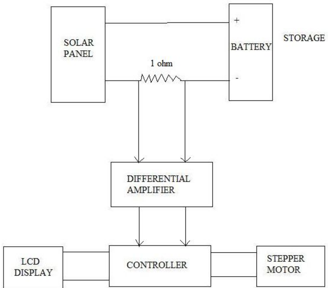
Figure 4.1: Block diagram
