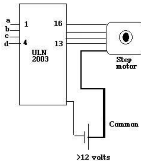
Figure2.8: Compact design
