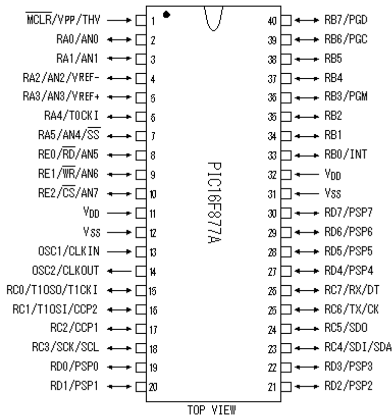
Figure 3.3: Pin Diagram
