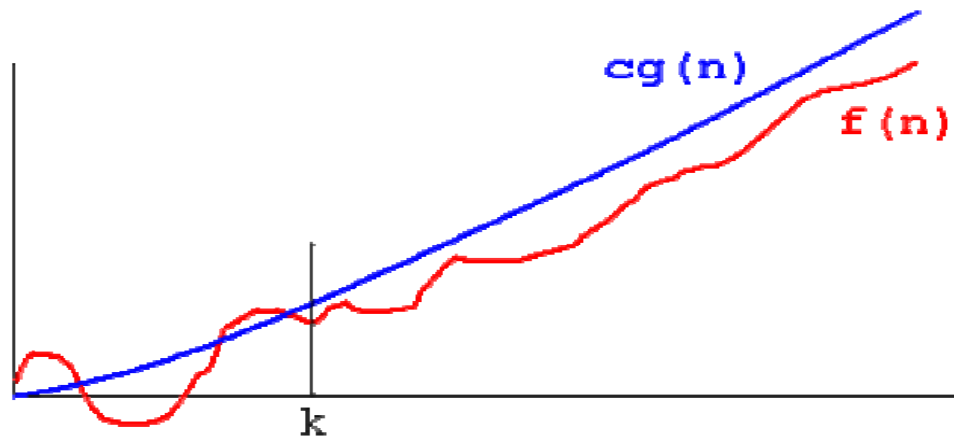
Figure 3.1: Big O Notation Graph
