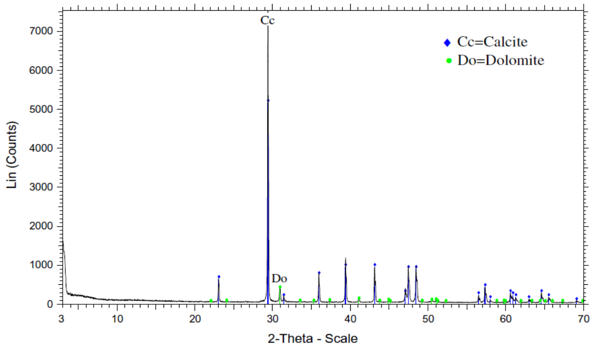
Fig. 1.2 : X-Ray Diffraction Pattern of Limestone Quarry Dust [Galetakis et. al. (2012)]
