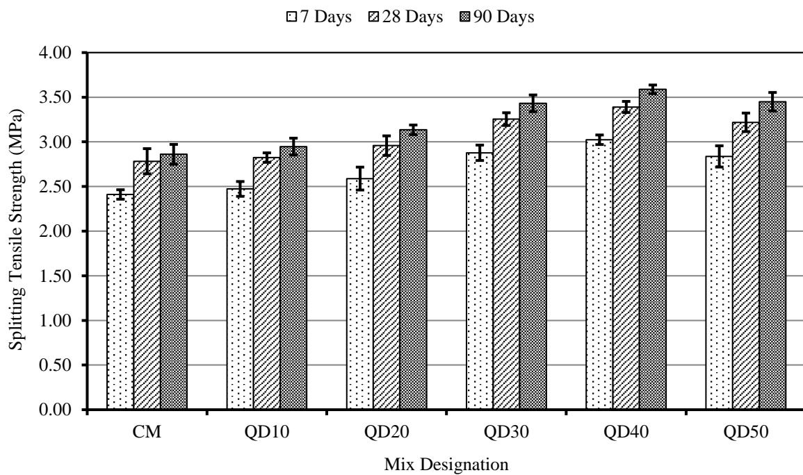
Figure 4.11 : Effect of Replacement of Natural Sand with Sandstone Quarry Dust on Splitting Tensile Strength of Concrete
