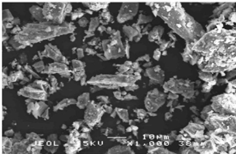
Figure 1.3 : SEM image of Granite Dust [Singh et. al.(2016)]
