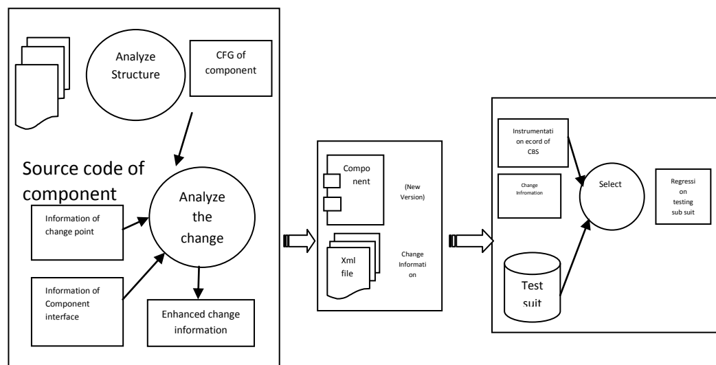
Fig. 7: Regression testing using enhanced change information [19]
