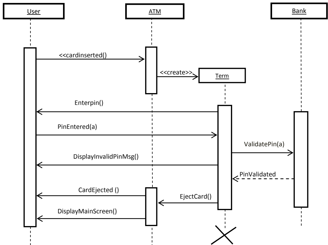
Fig. 33: Sequence Diagram of Invalid Pin of Original ATM System
