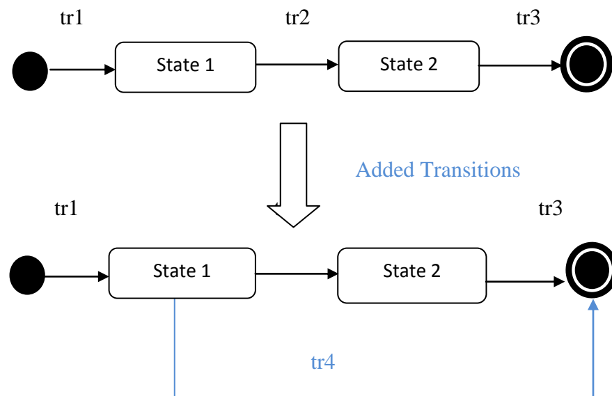
Fig. 15: Addition of a transition
