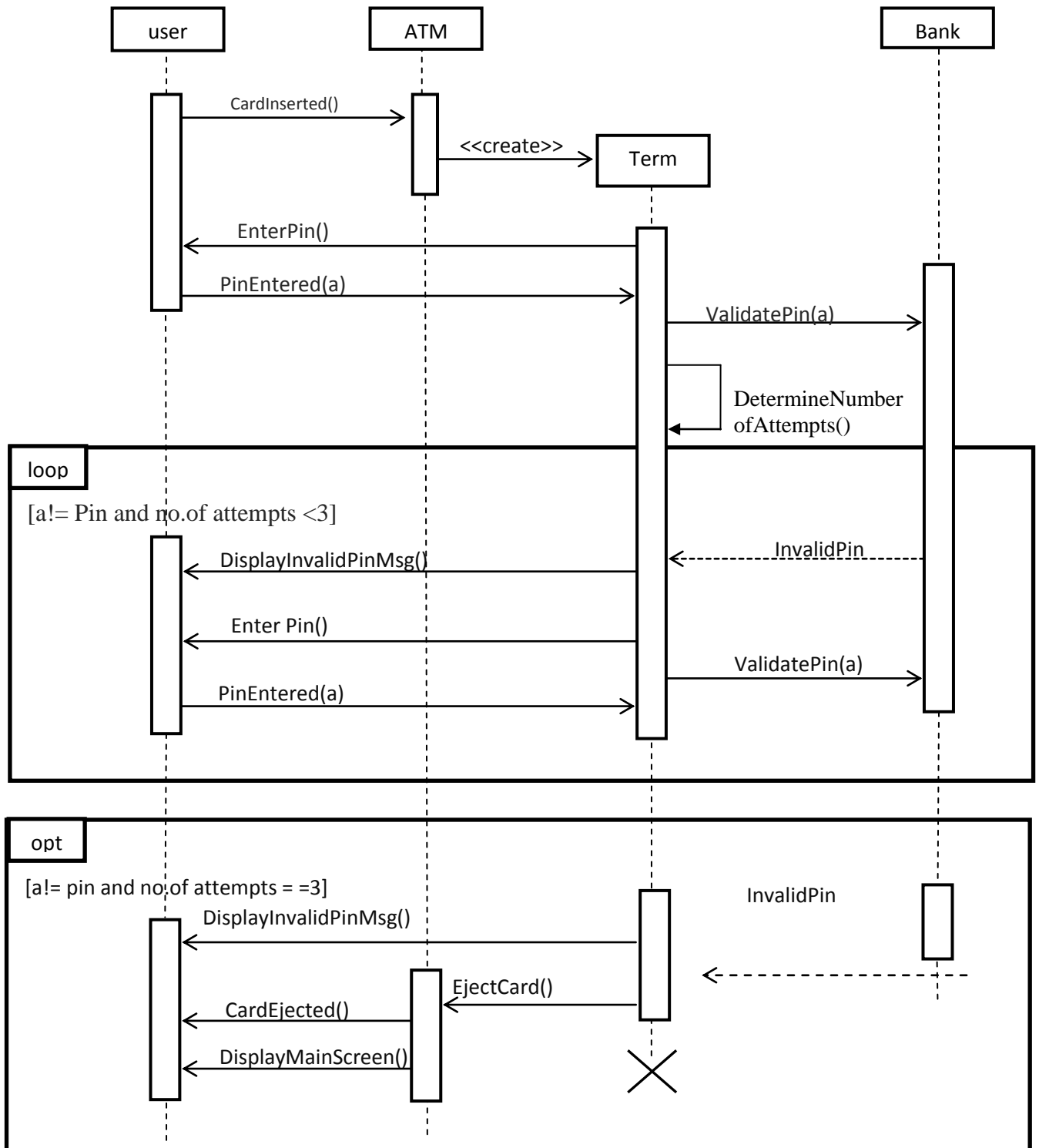
Fig. 34: Sequence Diagram of Invalid Pin of Modified ATM System
