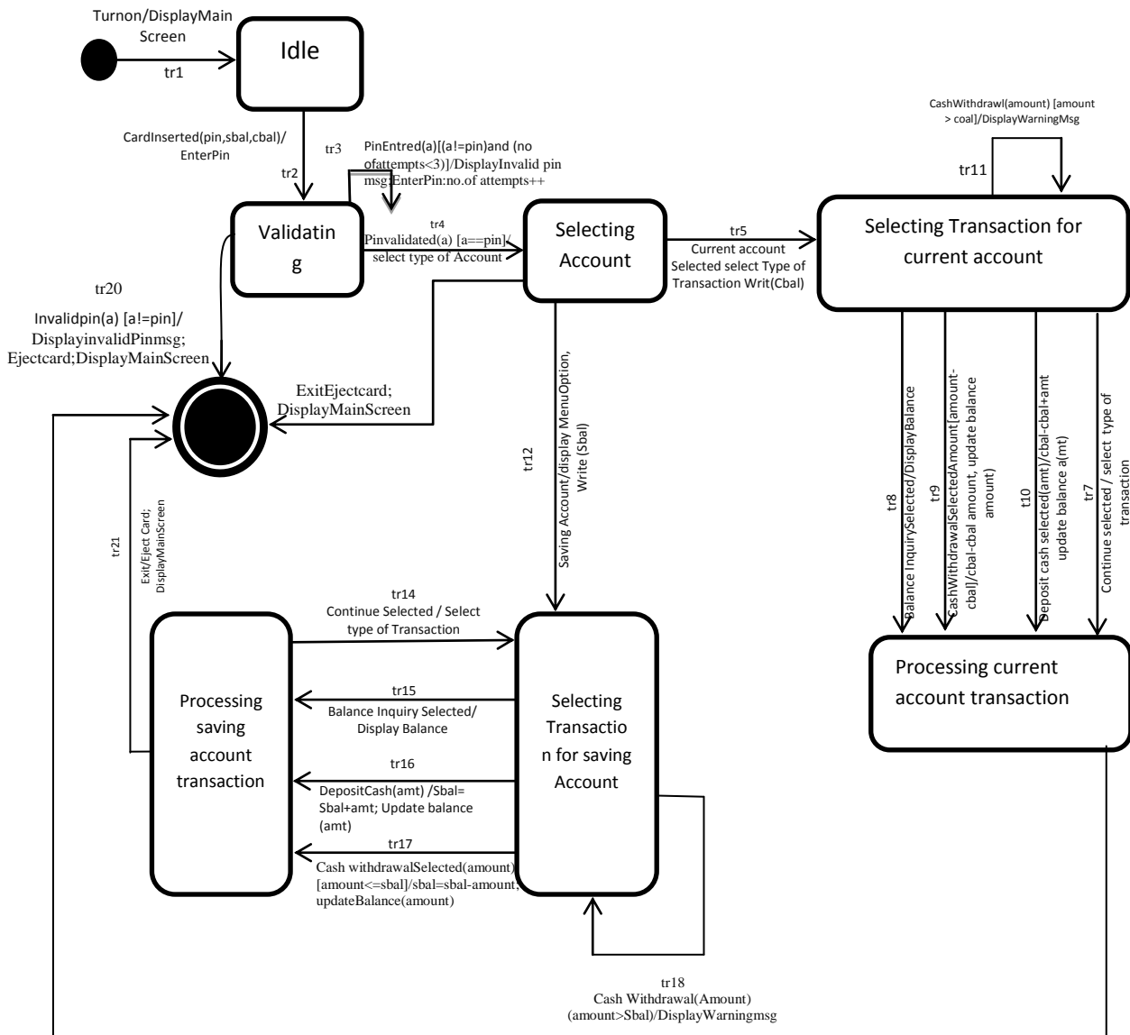
Fig. 31: State Chart Diagram of Modified ATM
