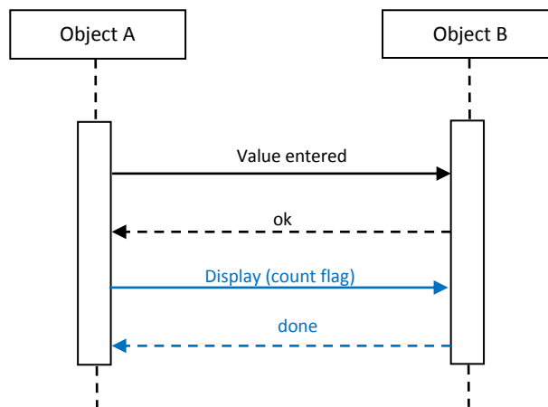
Sequence Diagram of Modified System
