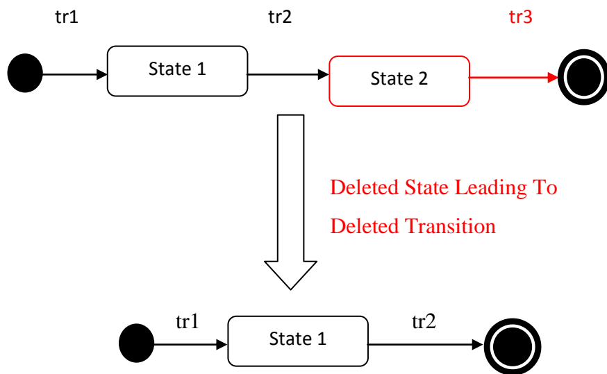
Fig. 14: Removal of a state
