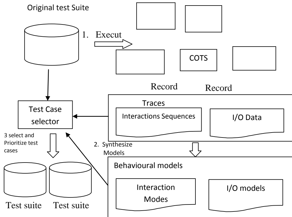
Fig. 8: Generation of compatibility and prioritized regression test suite [25]
