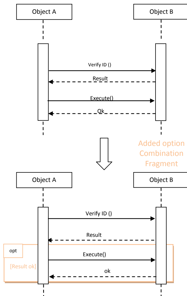
Fig. 25: Addition of Option Combination Fragment
