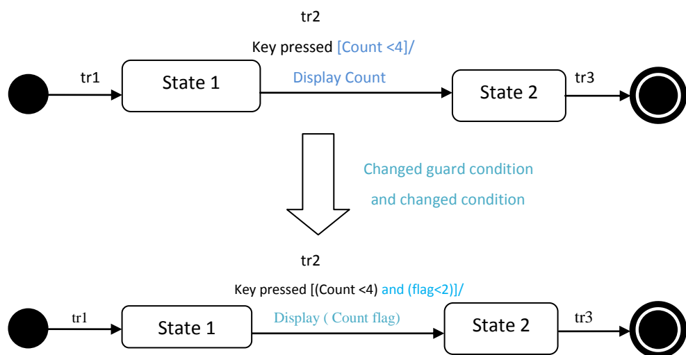
Fig. 27: change in the state chart diagram for system A.
