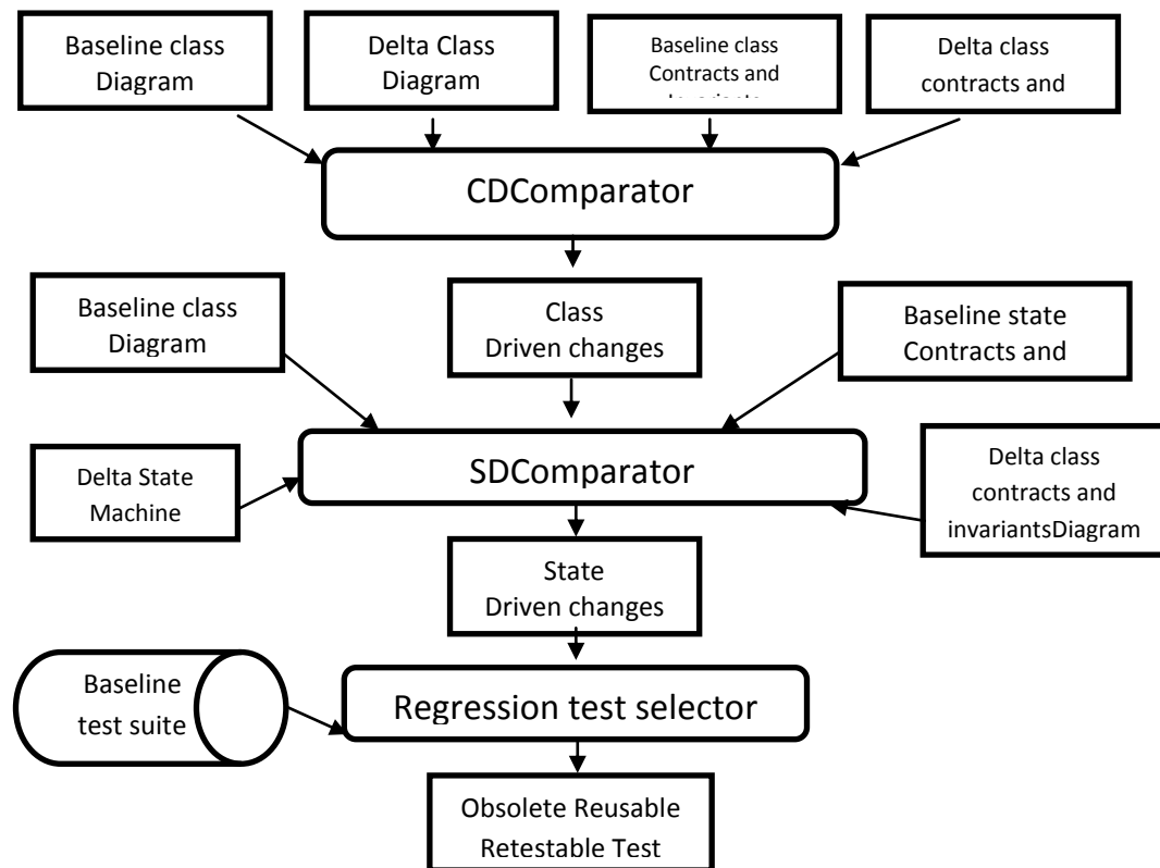
Fig: 9. State based regression testing [28]
