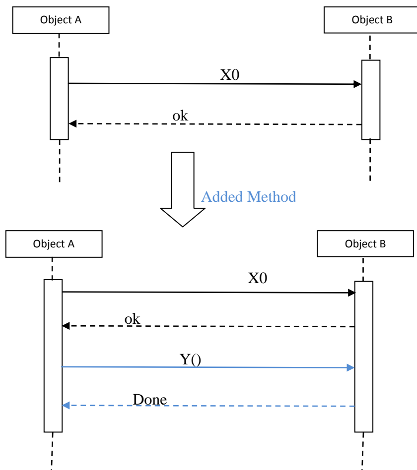
Fig.19: Addition of Method
