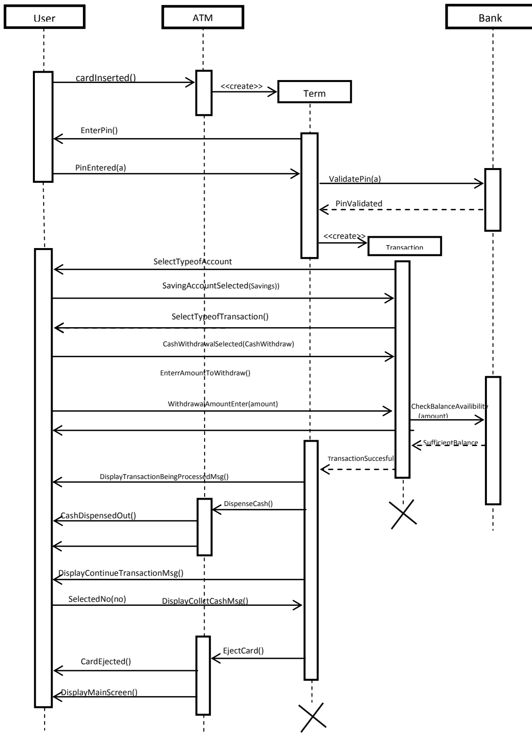
Fig. 35: Sequence Diagram of Cash Withdrawal from Savings of Original ATM System
