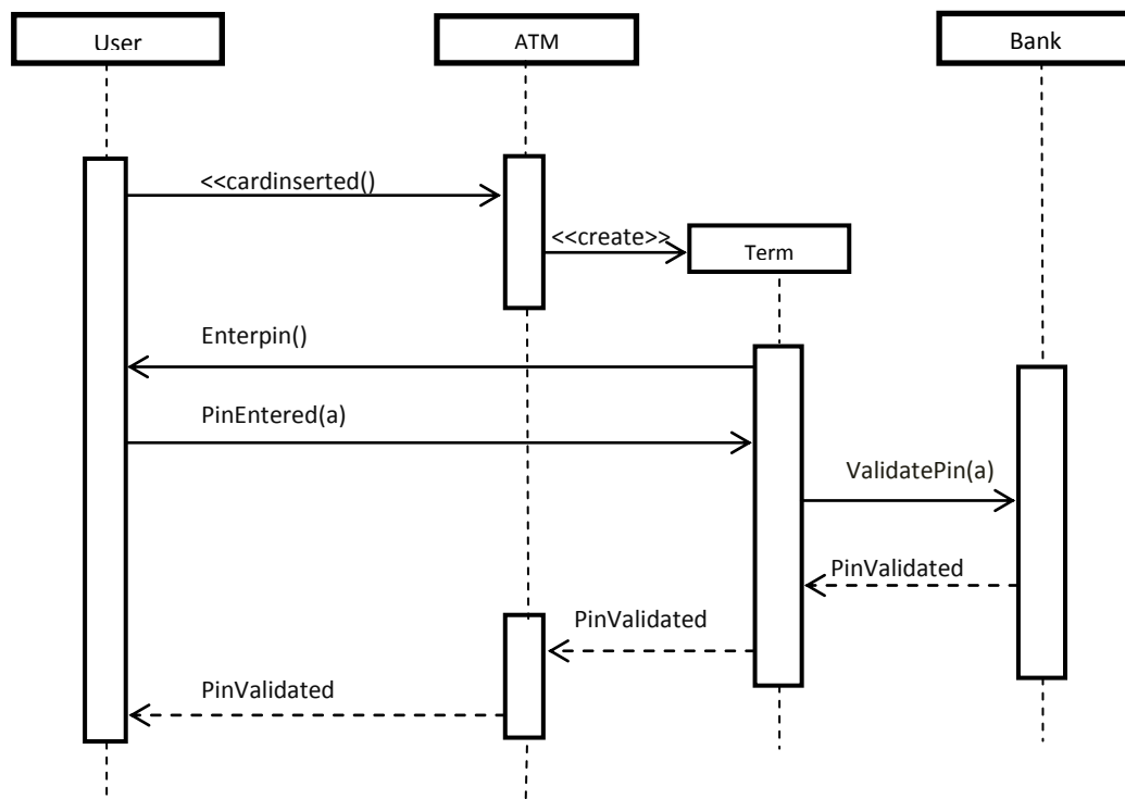
Fig. 32: Sequence Diagram of Valid Pin of ATM System
