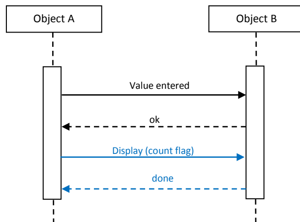
Sequence Diagram of original system
