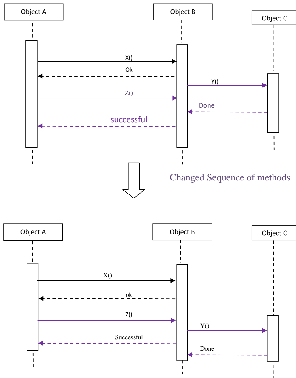
Fig.22: Modified Sequence of Methods
