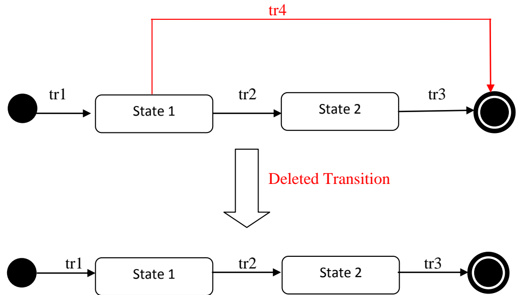
Fig . 16: Removal of a Transition
